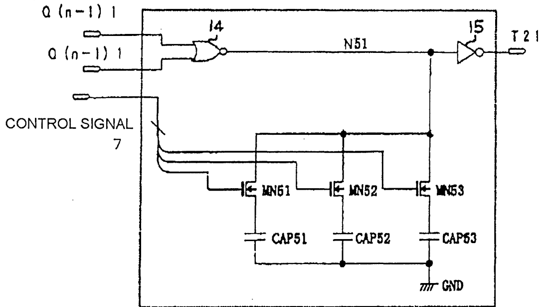
TIMING-DIFFERENCE DIVIDING CIRCUIT 4a1
