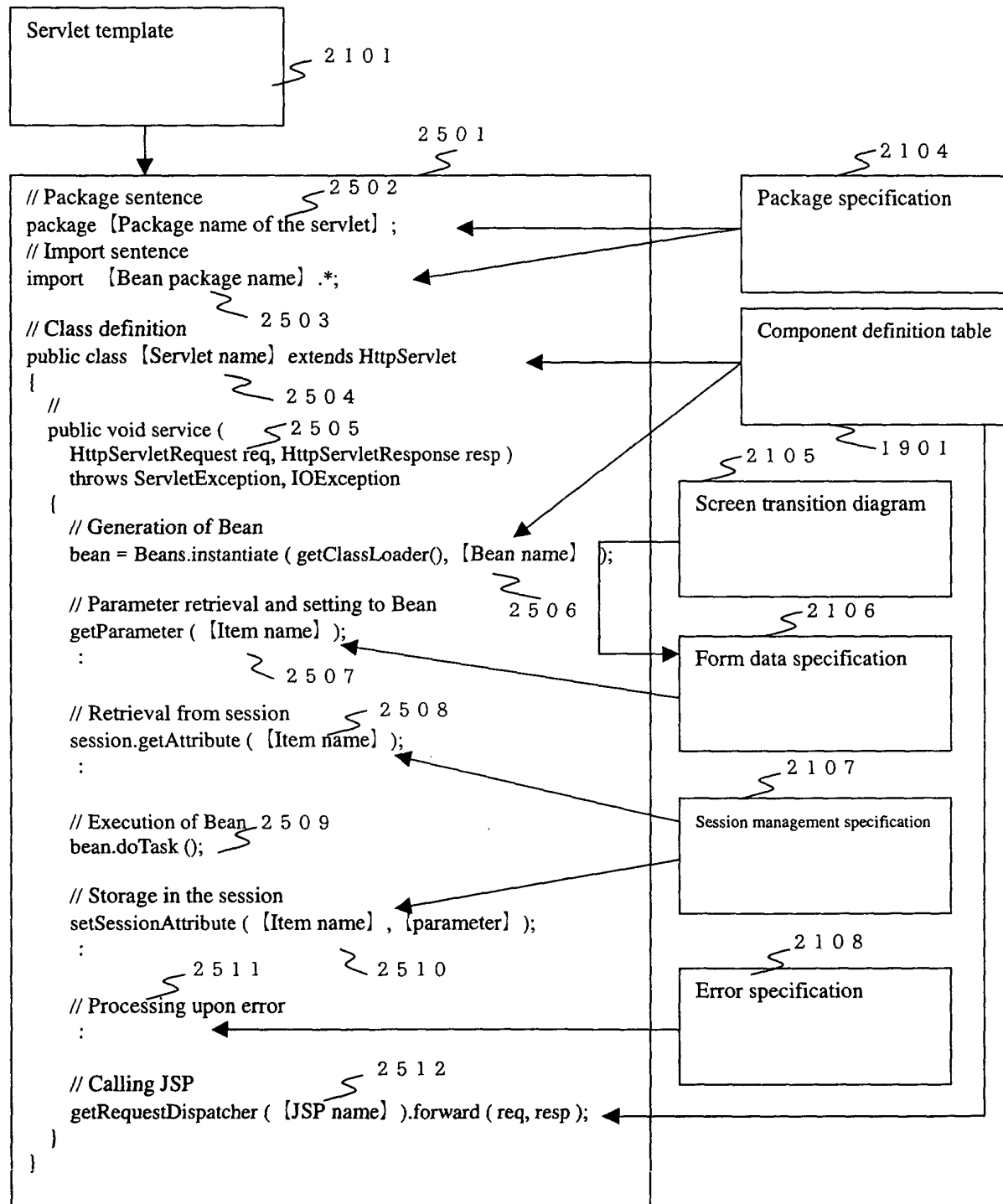
Fig.25 Example of generating a servlet source code
