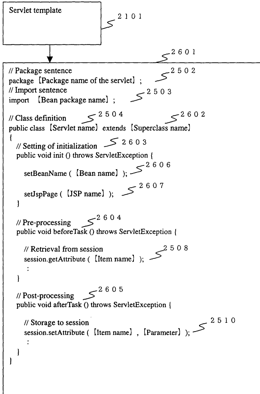
Fig.26 Generation of a servlet source code
