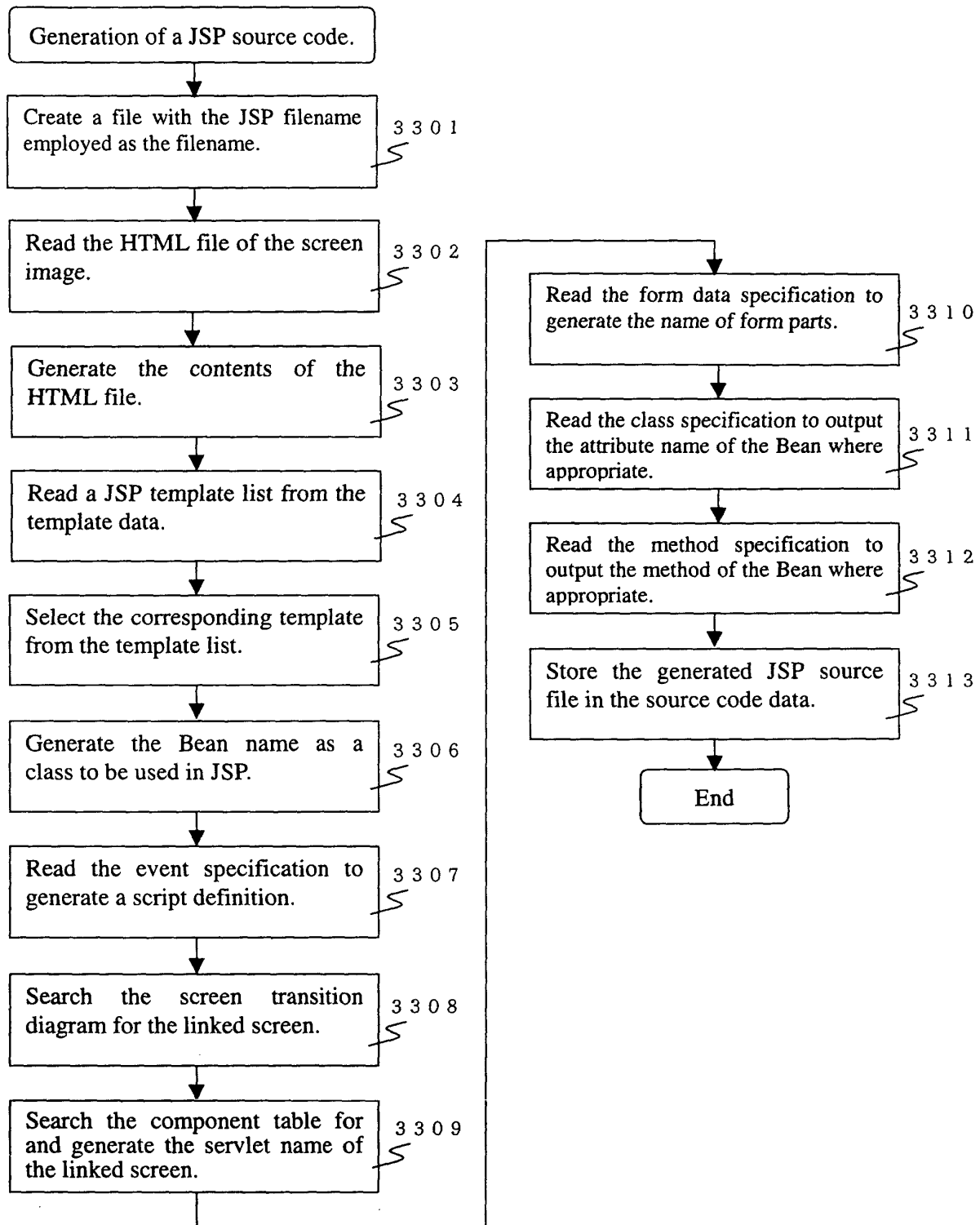
Fig.33 Flowchart for automatically generating a JSP source code
