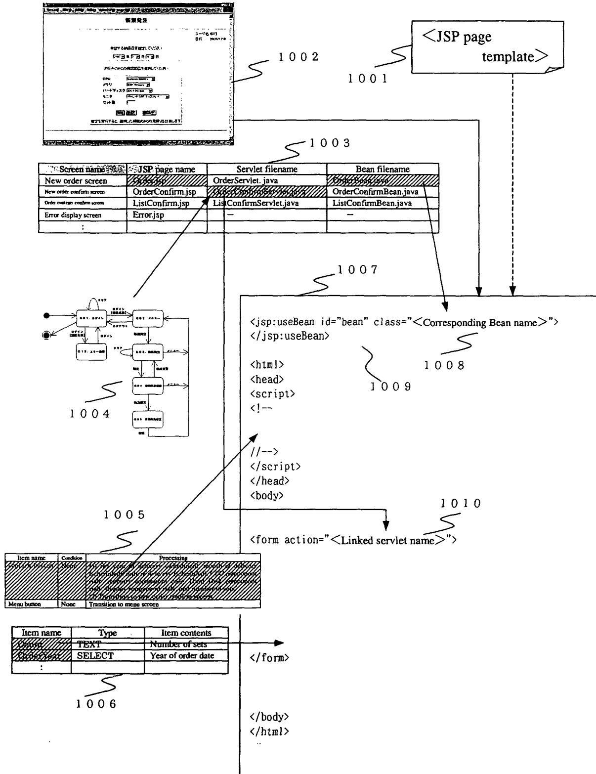
Fig.10 Generation of a JSP page source code
