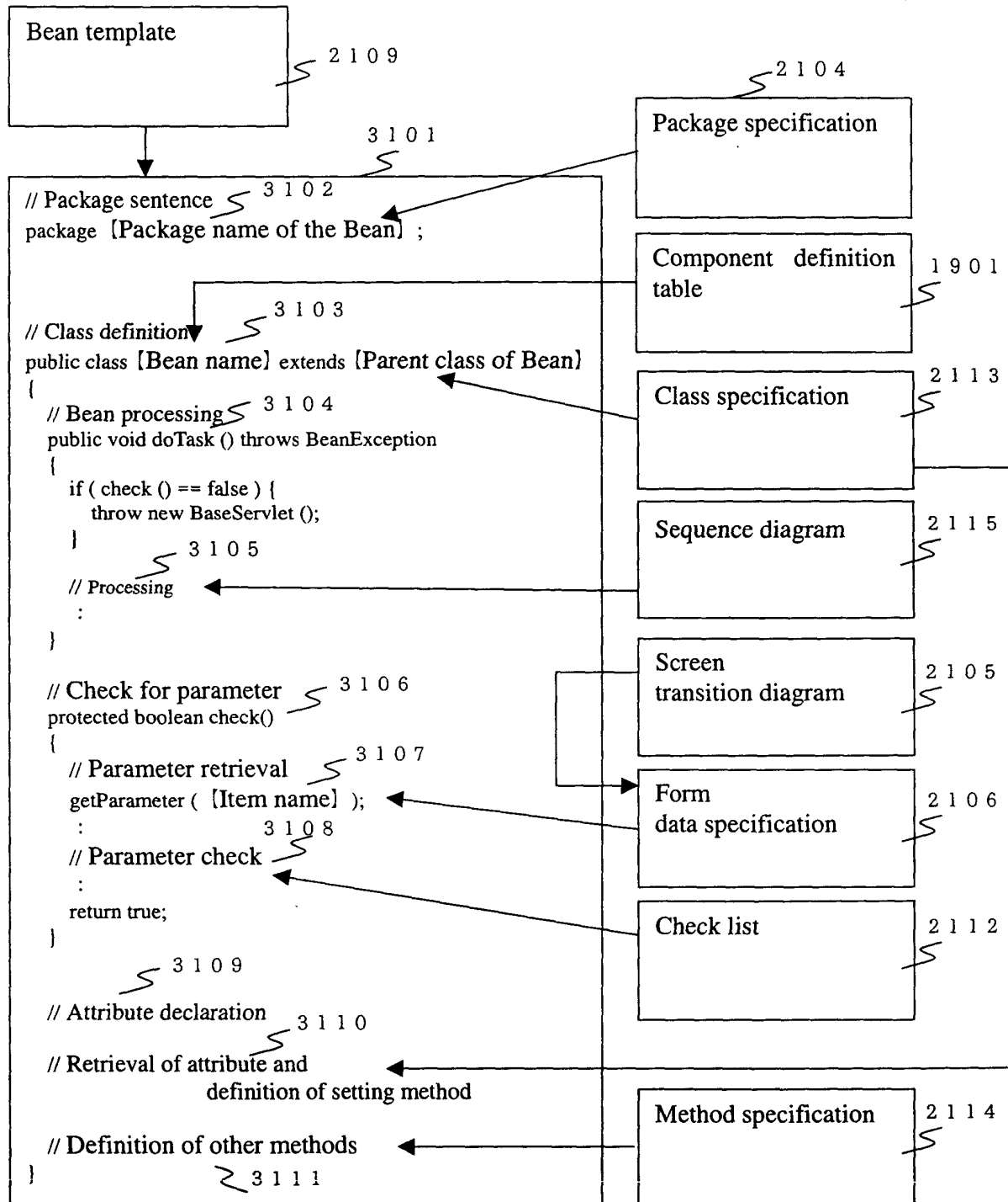
Fig.31 Example of generating a Bean source code
