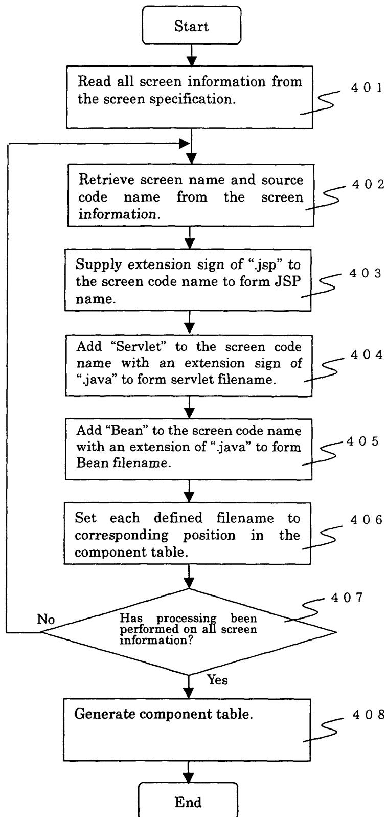
Fig.4 Flowchart for generating a component table
