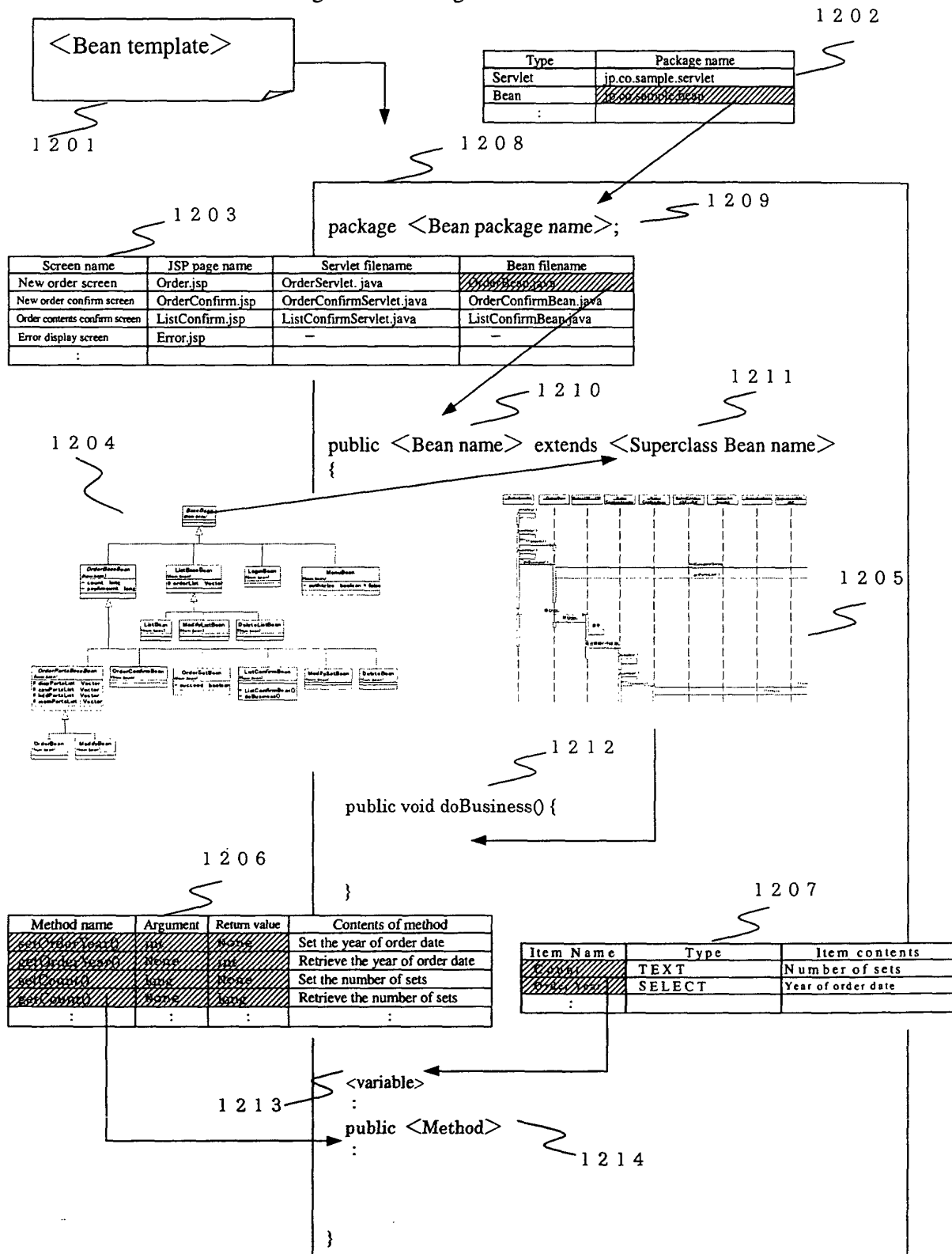
Fig.12 Generating Bean source code
