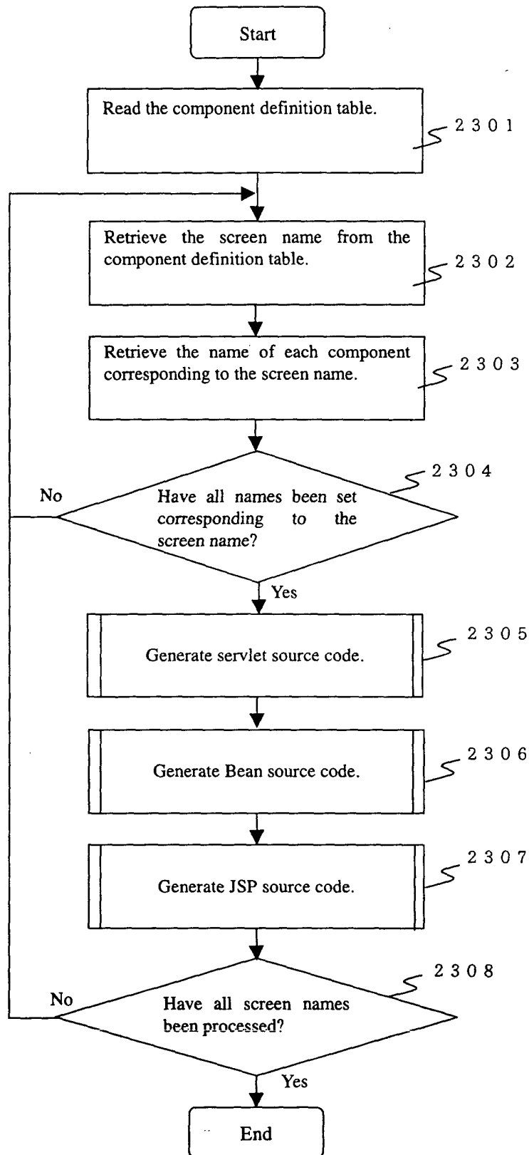
Fig.23 Flowchart for automatically generating a source code
