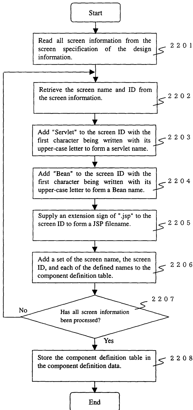
Fig.22 Flowchart for generating component definition table
