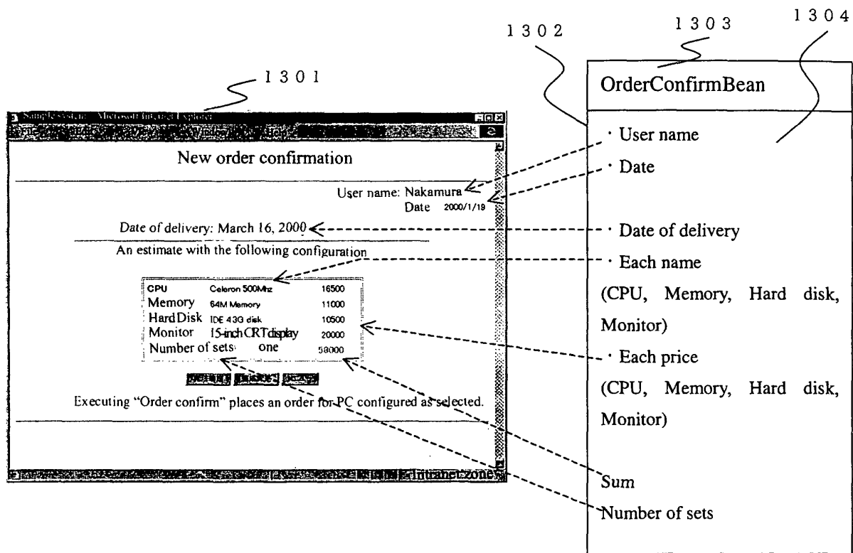
Fig.13 Relationship between screen information and Bean
