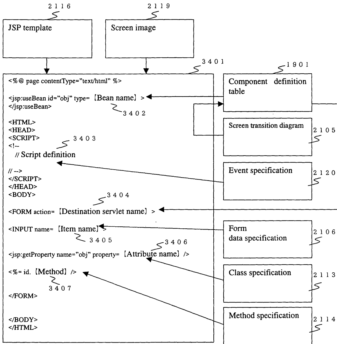
Fig.34 Example of generating a JSP source code
