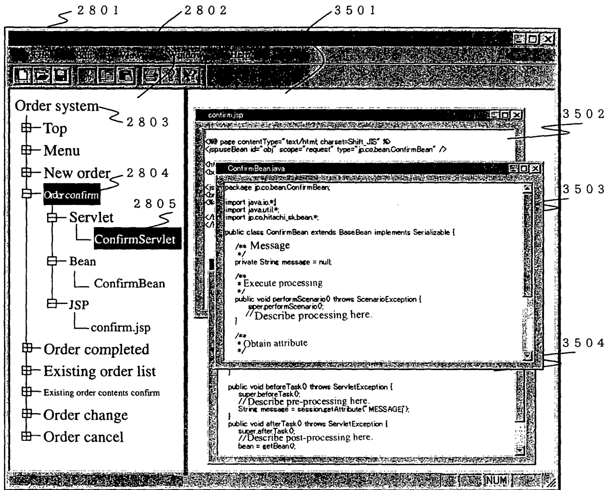
Fig.35 Image of editing source codes
