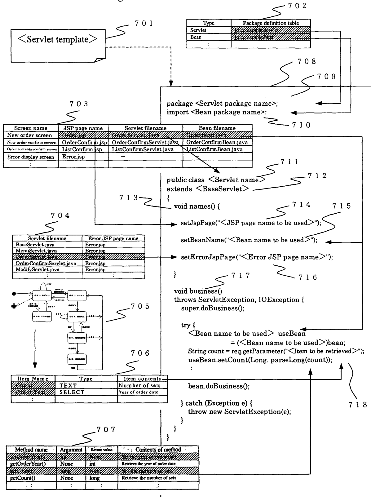
Fig.7 Generation of servlet source code
