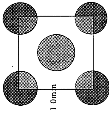
Fig. 2 0.5mm(diameter) In a staggered arrangement pitch (Example 5)
