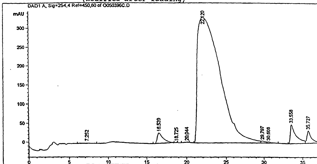
Figure 31 Liquid Chromatographic Separation of Eupatorium odoratum Antileishmanial Fraction E00 60-104.
