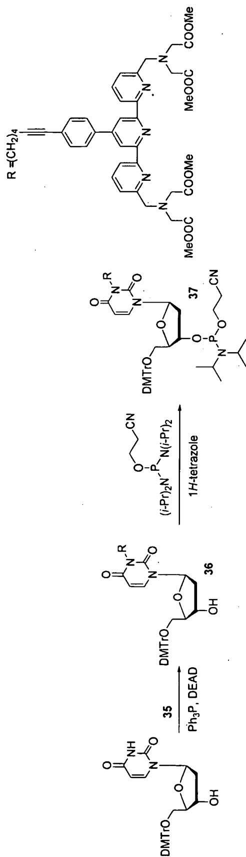
SCHEME 7B
