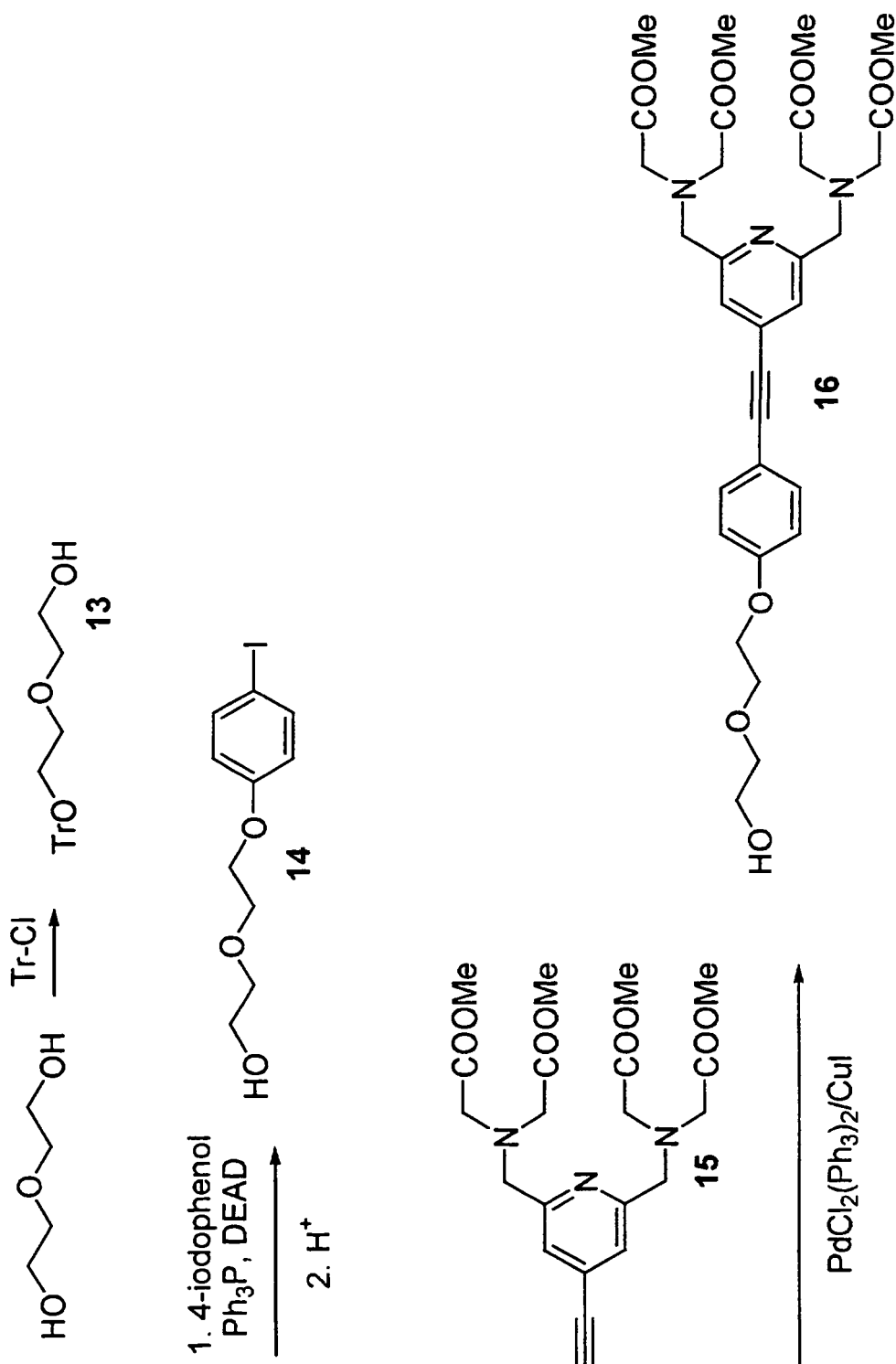
SCHEME 5A
