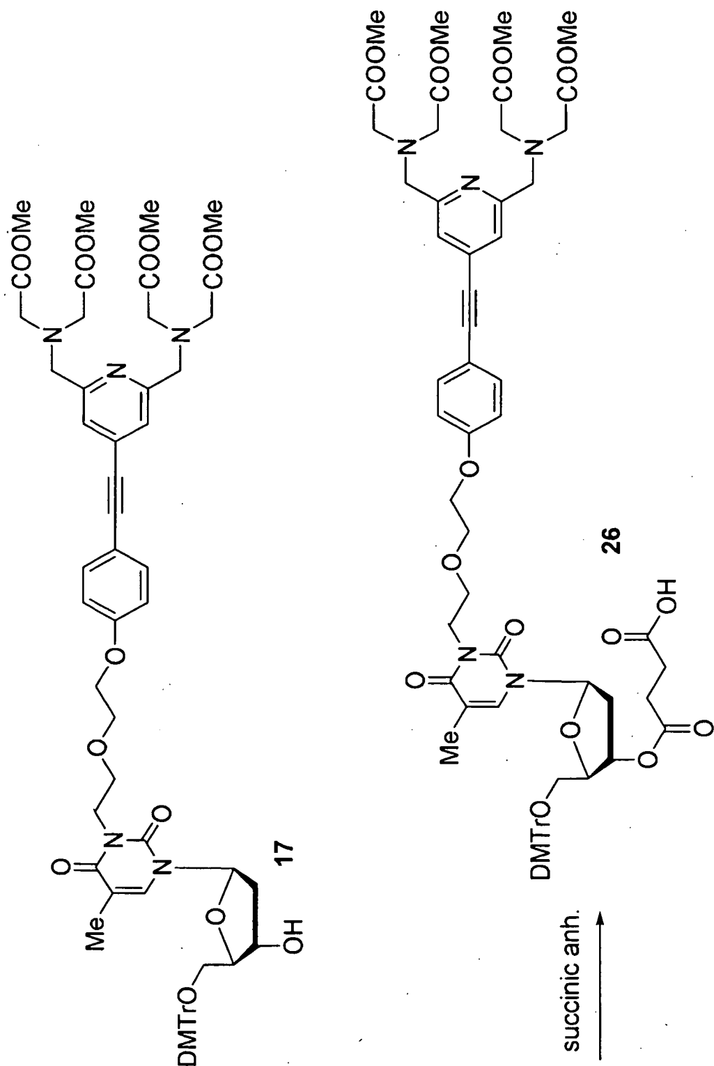
SCHEME 6A
