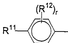
Structural formula (3)
