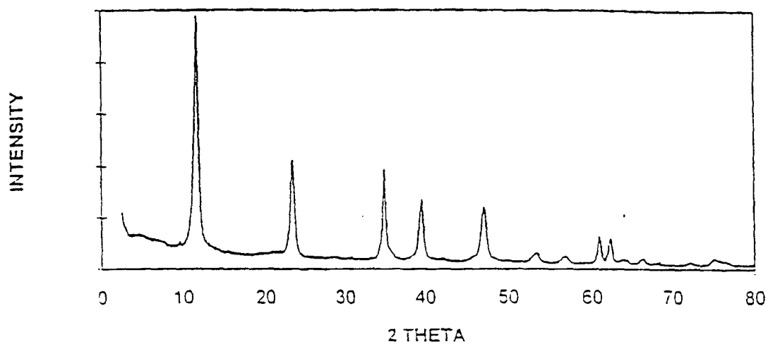
FIGURE 2: X-RAY DIFFRACTION PATTERN FOR COMMERCIAL ANIONIC CLAY
