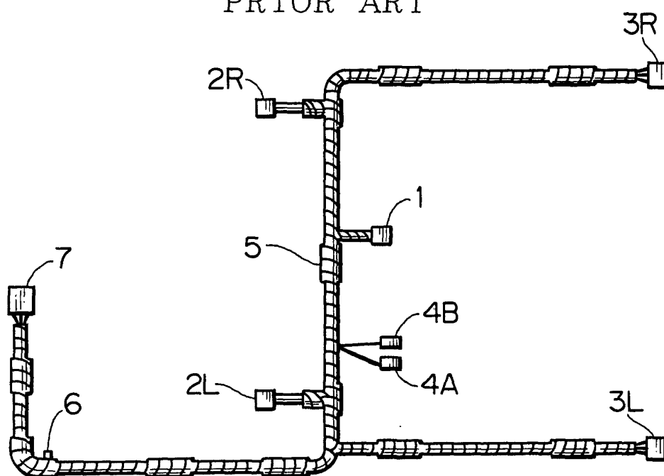
FIG. 8 PRIOR ART
