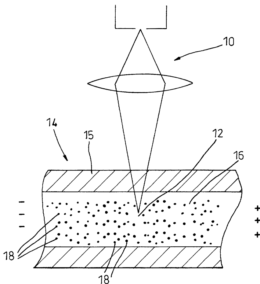
Fig. 1 (PRIOR ART)
