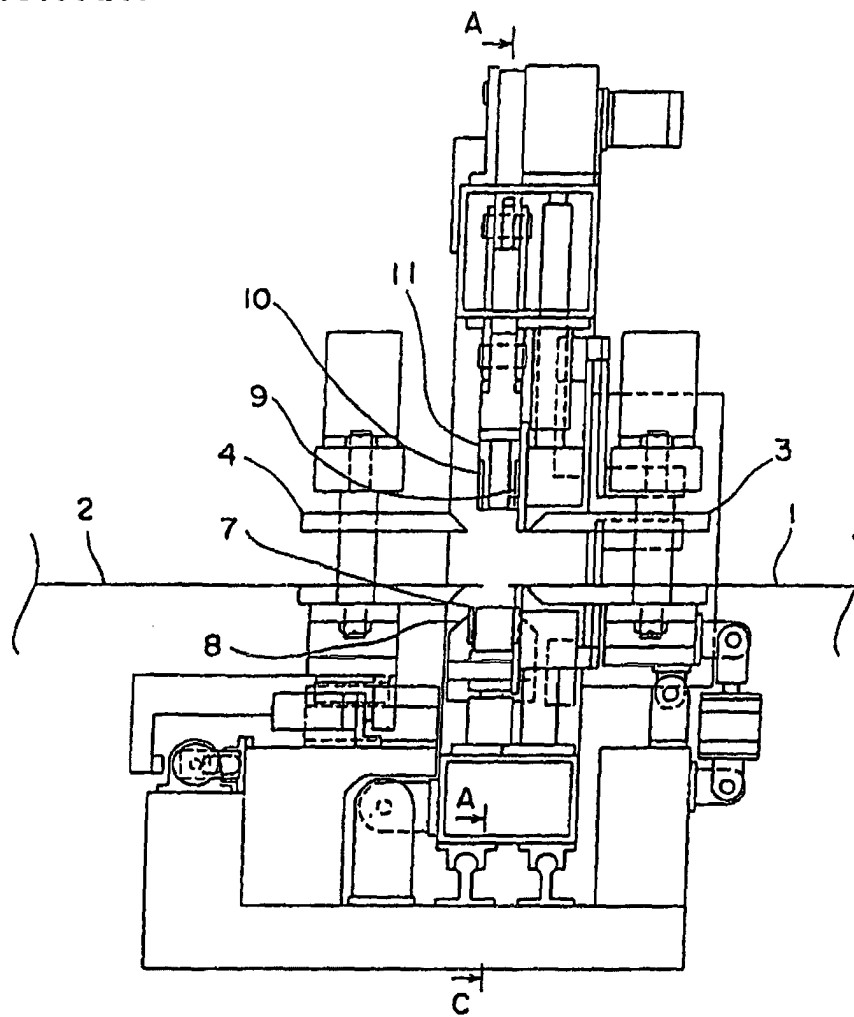
FIG. 12 PRIOR ART
