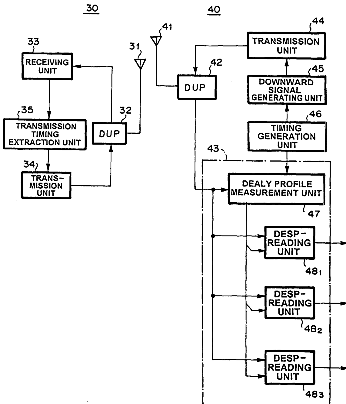
FIG.6 PRIOR ART
