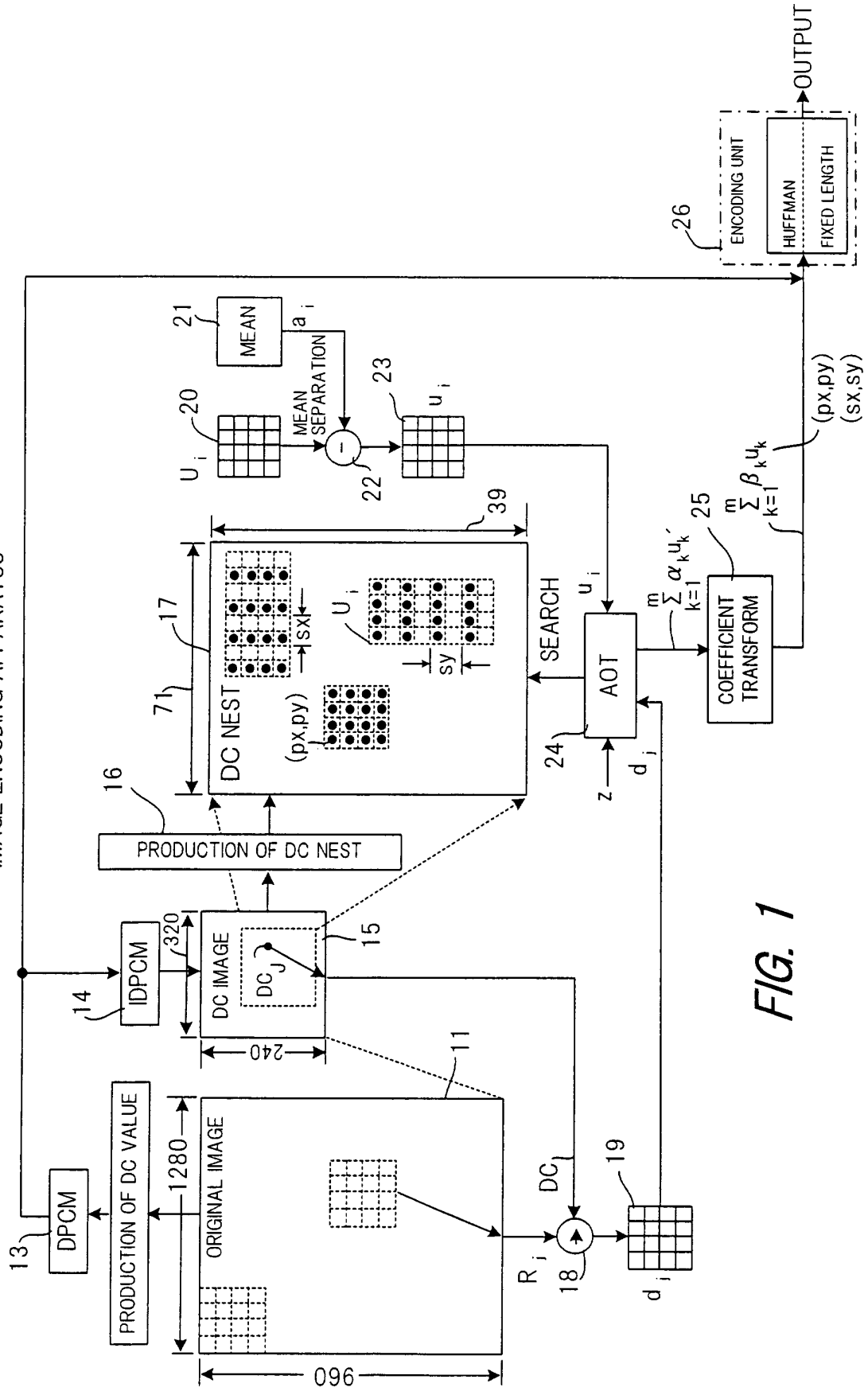
BLOCK DIAGRAM OF CONVENTIONAL IMAGE ENCODING APPARATUS
