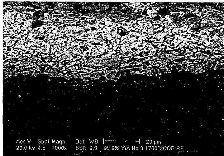
Surface of 1700°C Co-sintered product (×1000)
