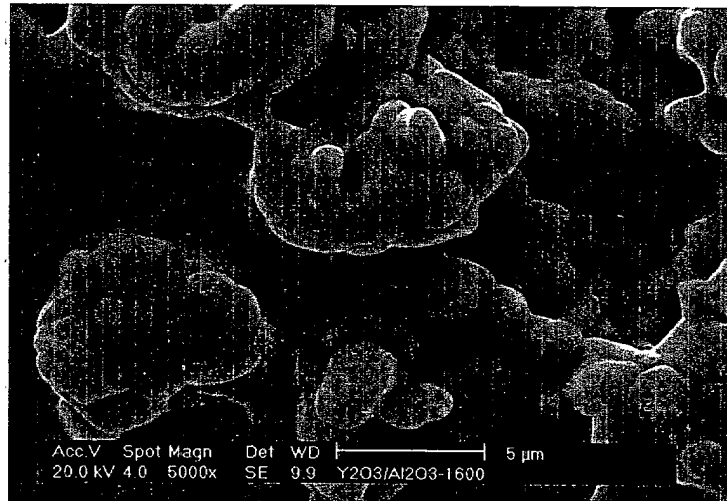
Surface of 1600°C×3h Co-sintered product (×5000)
