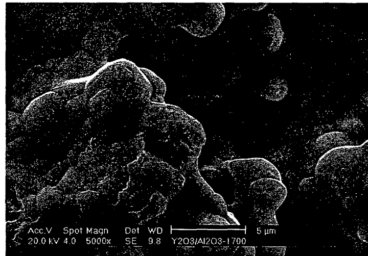
Surface of 1700°C×3h Co-sintered product (×5000)
