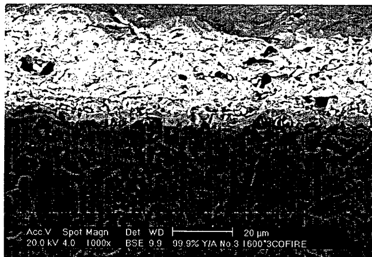
Surface of 1600°C Co-sintered product (×1000)
