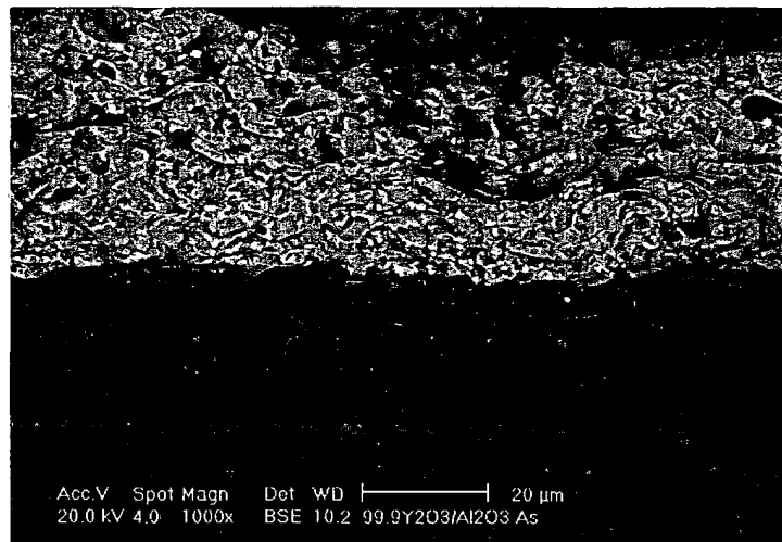
Section of 99.9% Y_2O_3 sprayed product ( \times 1000 )
