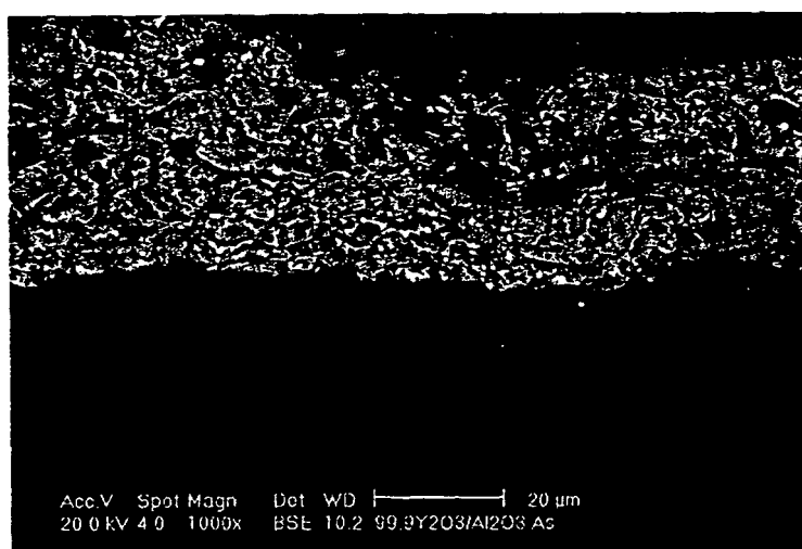
Section of 99.9% Y_2O_3 sprayed product ( \times 1000 )
