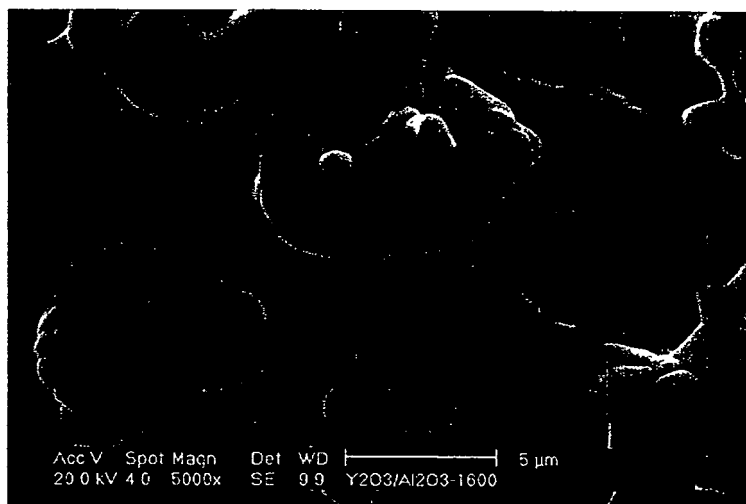
Surface of 1600°C X 3h Co-sintered product (X5000)
