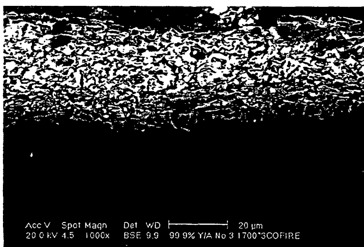
Surface of 1700°C Co-sintered product (×1000)
