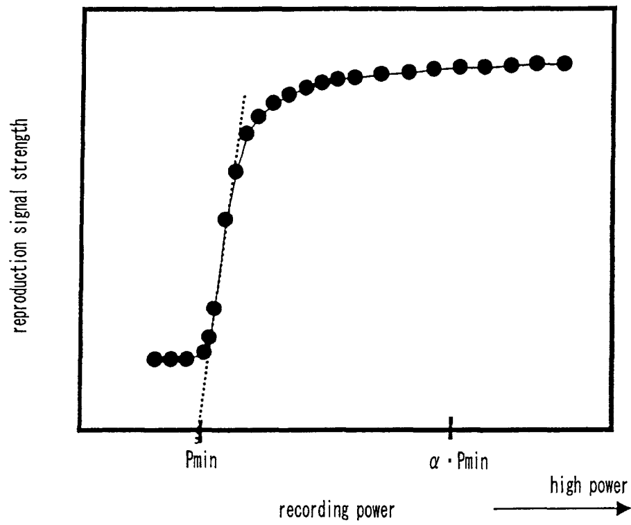
FIG. 19 PRIOR ART
