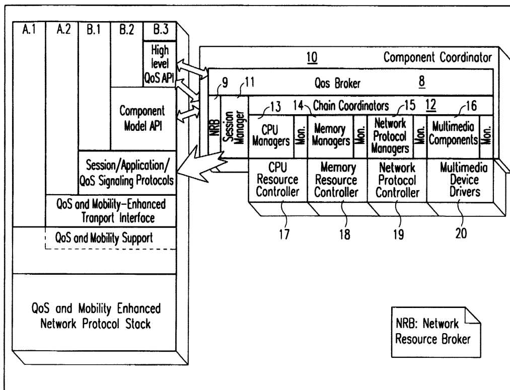
End System Reference Architecture
