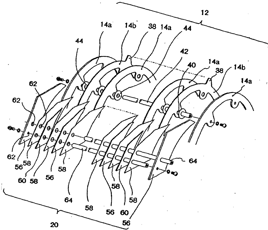
FIG. 10 PRIOR ART
