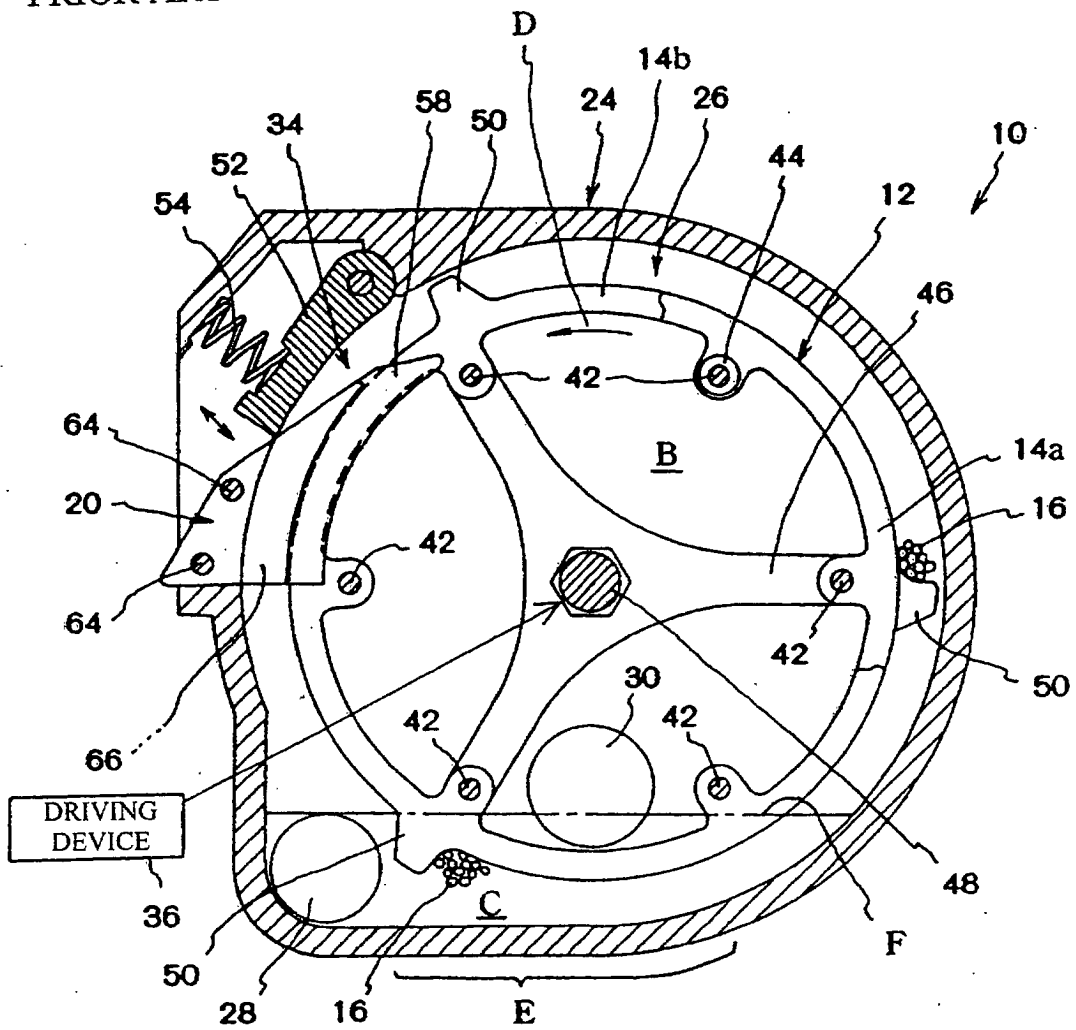
FIG. 8 PRIOR ART
