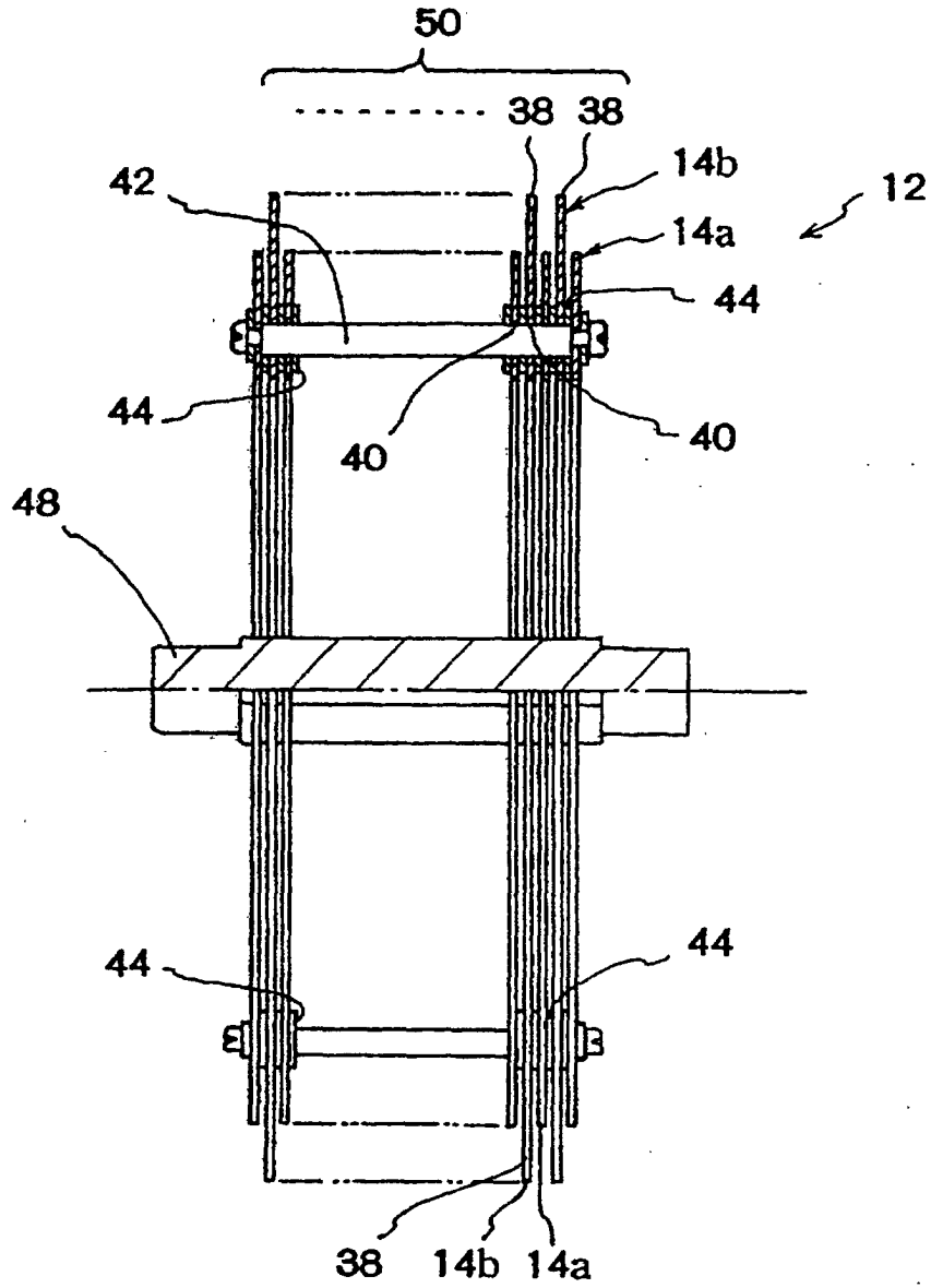
FIG. 9 PRIOR ART
