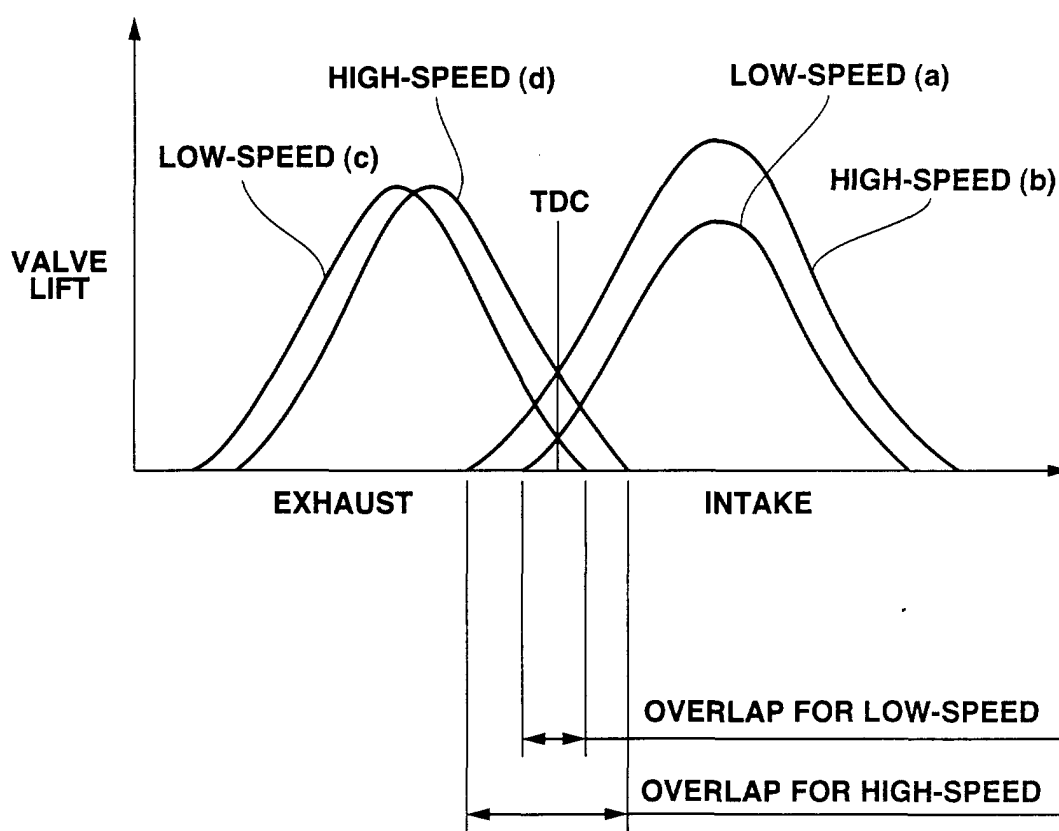
FIG.12 (RELATED ART)
