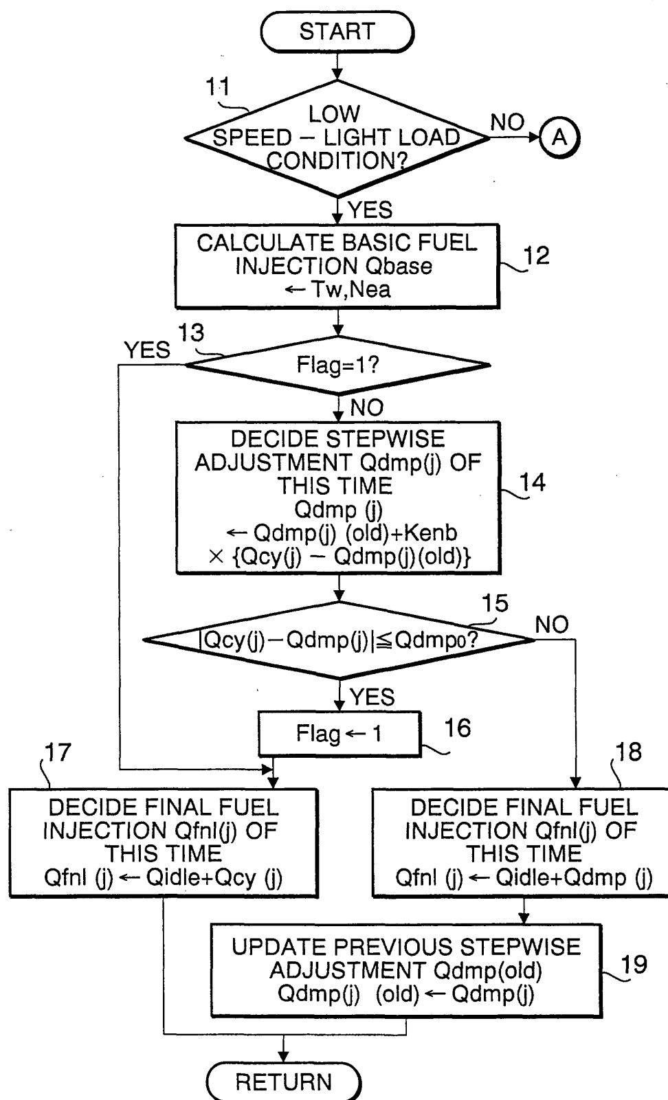
FLOWCHART OF FUEL INJECTION DETERMINATION (1)
