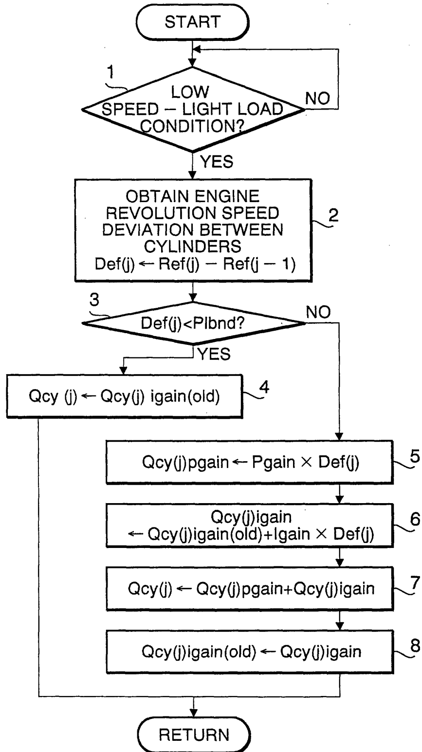
FLOWCHART OF FUEL INJECTION ADJUSTMENT
