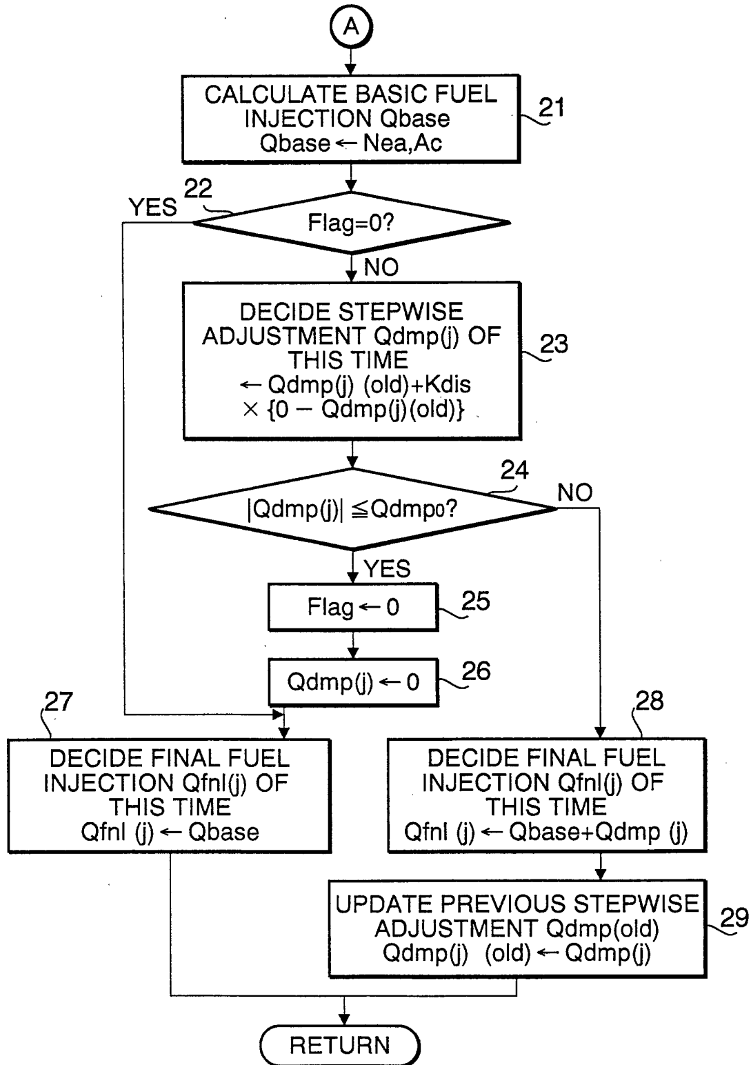
FLOWCHART OF FUEL INJECTION DETERMINATION (2)
