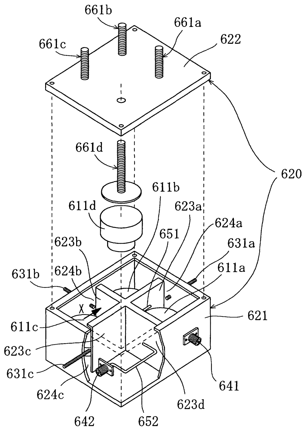
FIG. 24 PRIOR ART
