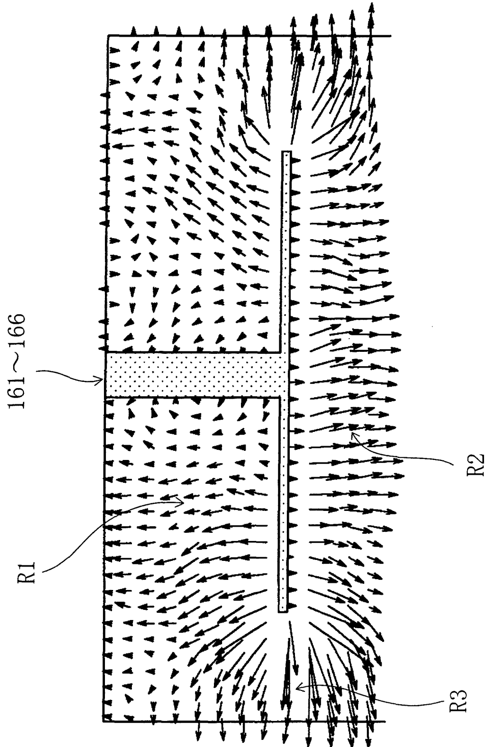
FIG. 22 PRIOR ART
