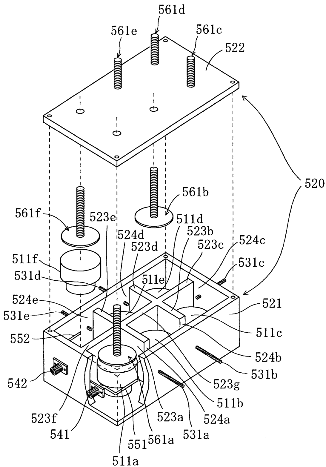
FIG. 21 PRIOR ART
