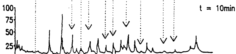
(PhyM) ApN → UpN → FIG. 77D
