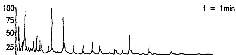
(RNase T 1 ) GpN → FIG. 77A
