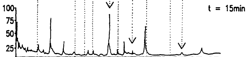
(U 2 ) ApN → FIG. 77C
