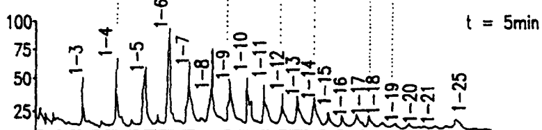
(ALKALINE HYDROLYSIS) FIG. 77B
