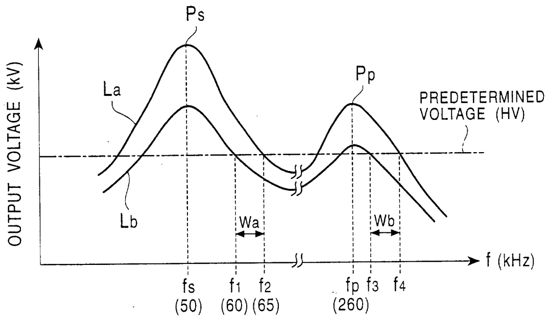
FIG. 7 PRIOR ART
