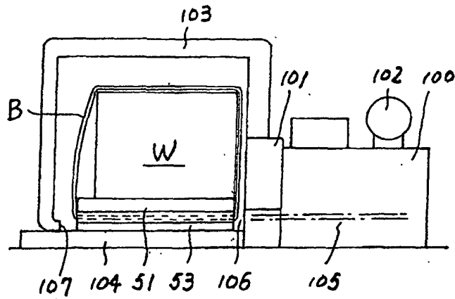
FIG. 18 PRIOR ART
