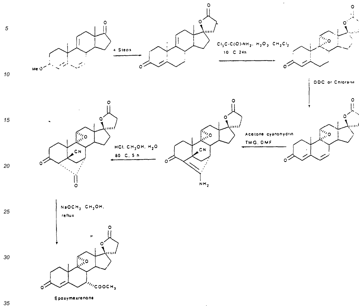
Scheme 5
