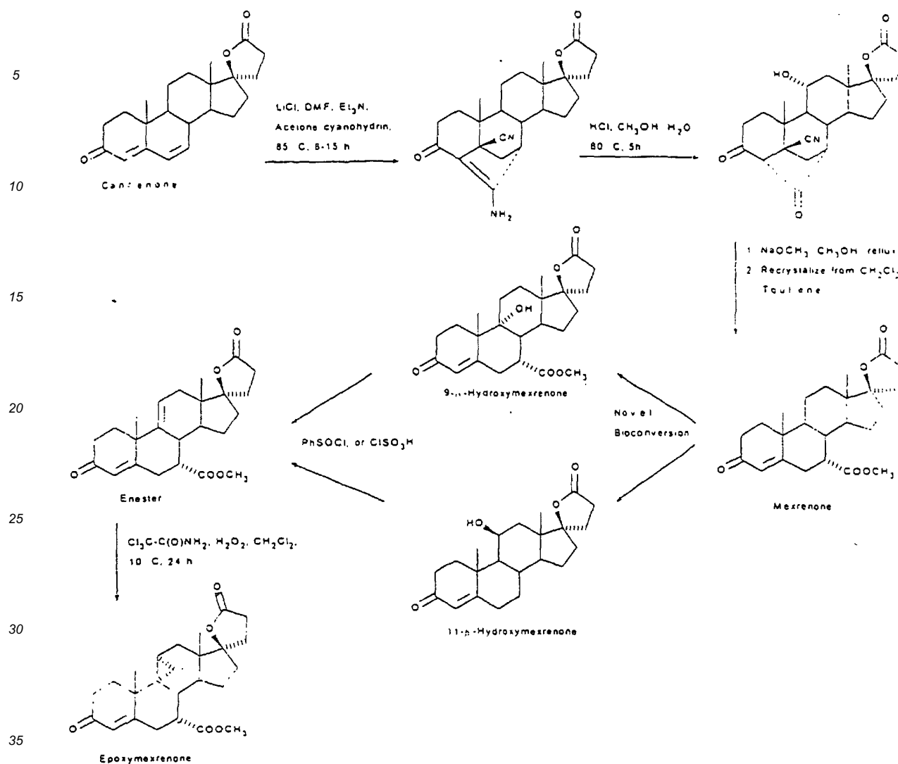
Scheme 3
