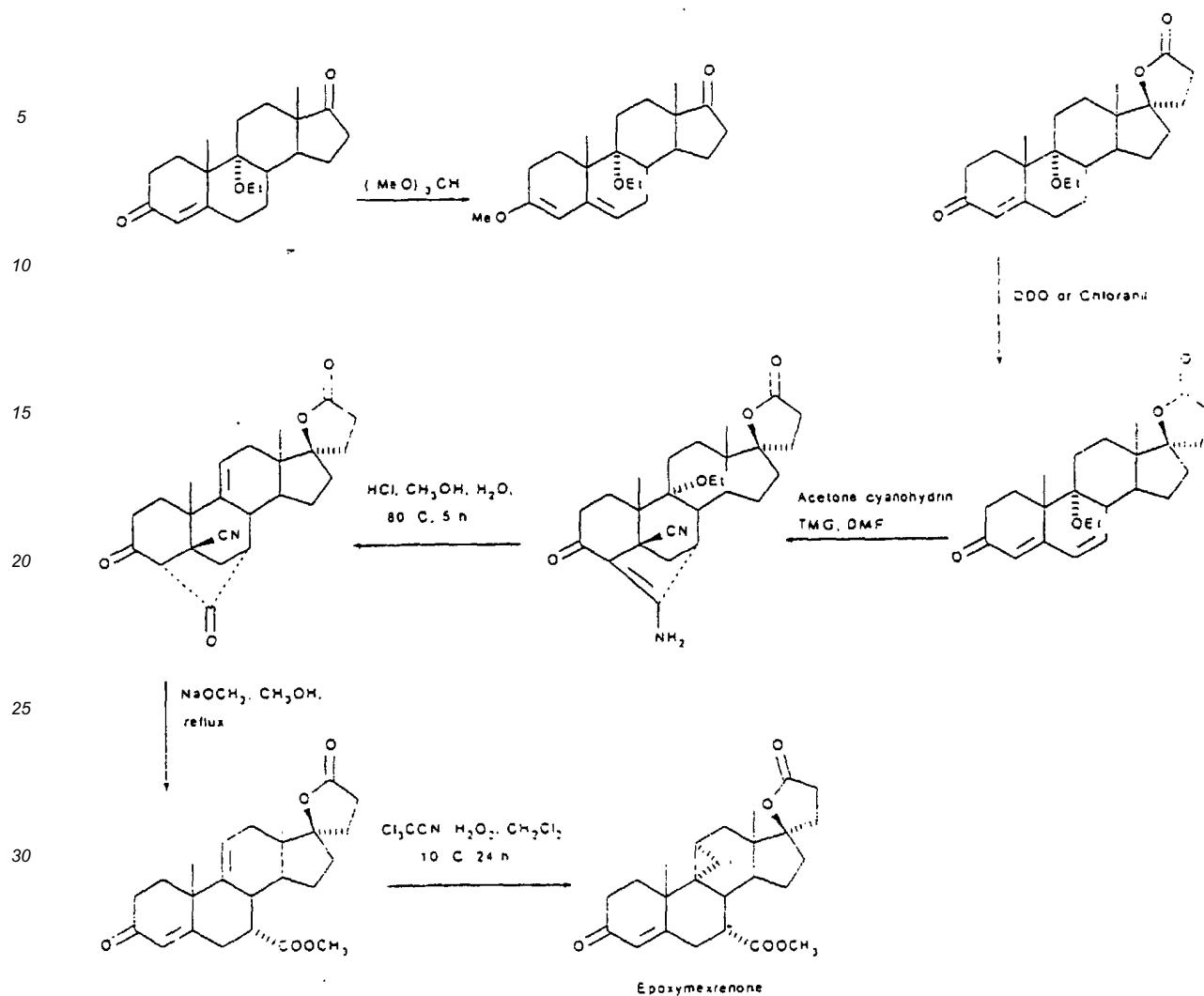
Scheme 6
