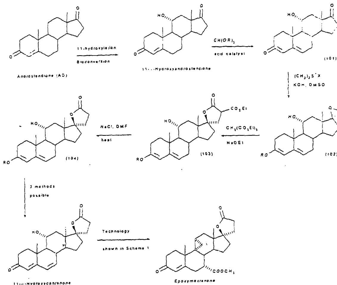
Scheme 7
