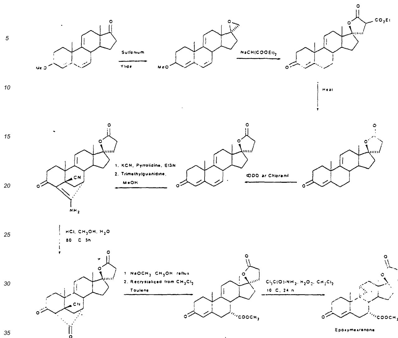
Scheme 4
