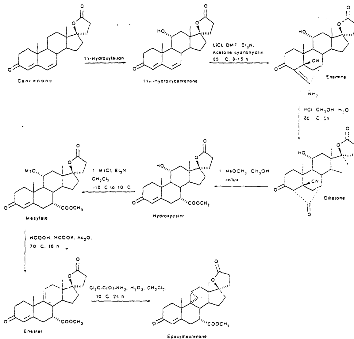
Scheme 2
