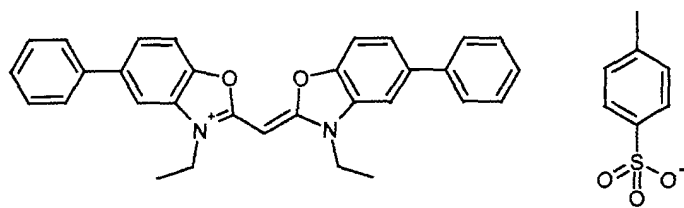
Dye (II.18)
