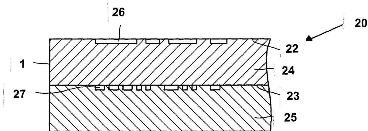
FIG. 2 (PRIOR ART)
