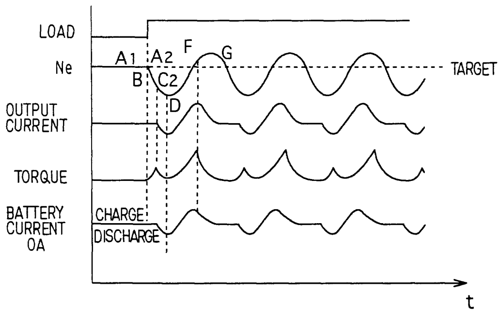
FIG. 9 PRIOR ART
