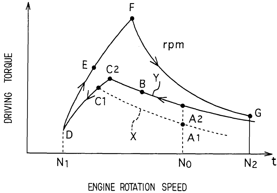
FIG. 8 PRIOR ART
