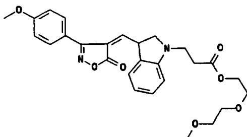
Compound F
