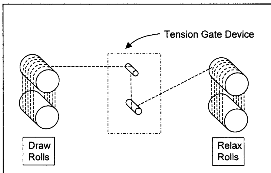
Configuration for Two-Roll Tension Gate Device
