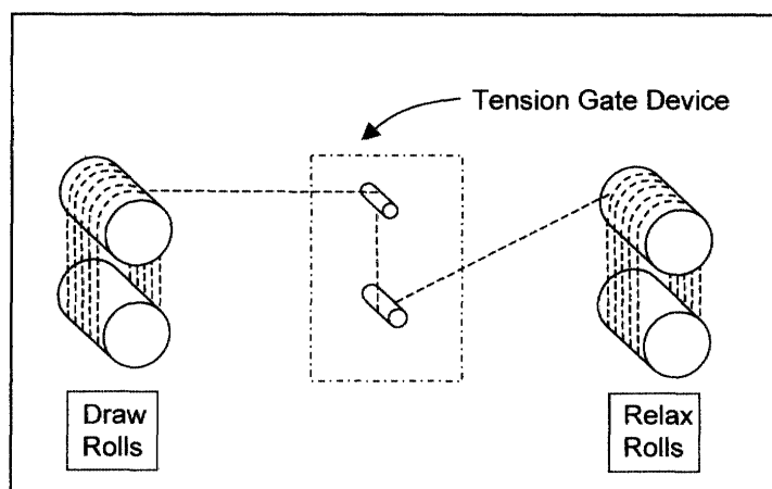
Configuration for Two-Roll Tension Gate Device
