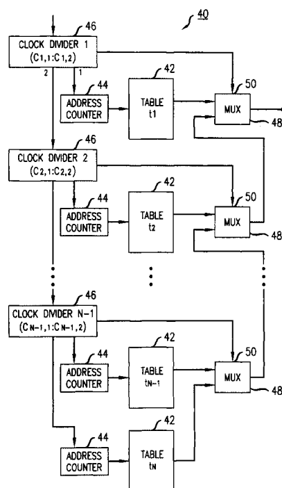
FIG. 4 RECURSIVE IMPLEMENTATION OF GRANT GENERATOR USING MULTI-TABLES
