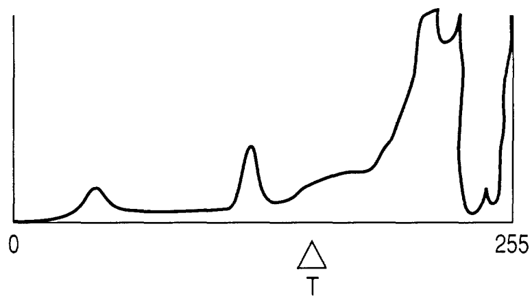
BRIGHTNESS HISTOGRAM
