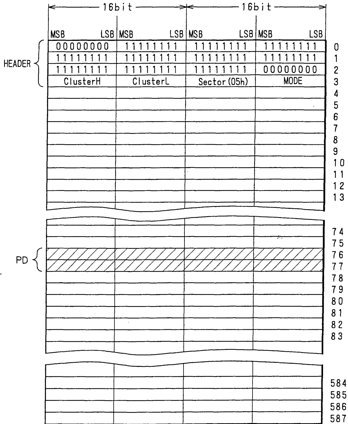
U-TOC SECTOR 5
