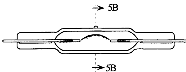
FIGURE 5 PRIOR ART
