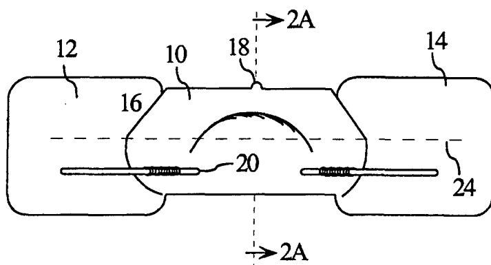
FIGURE 2 PRIOR ART
