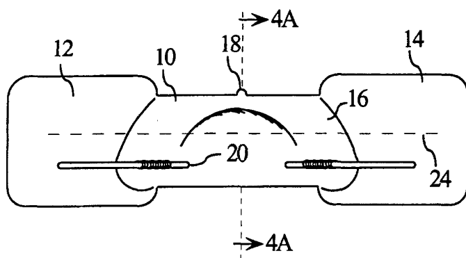
FIGURE 4 PRIOR ART
