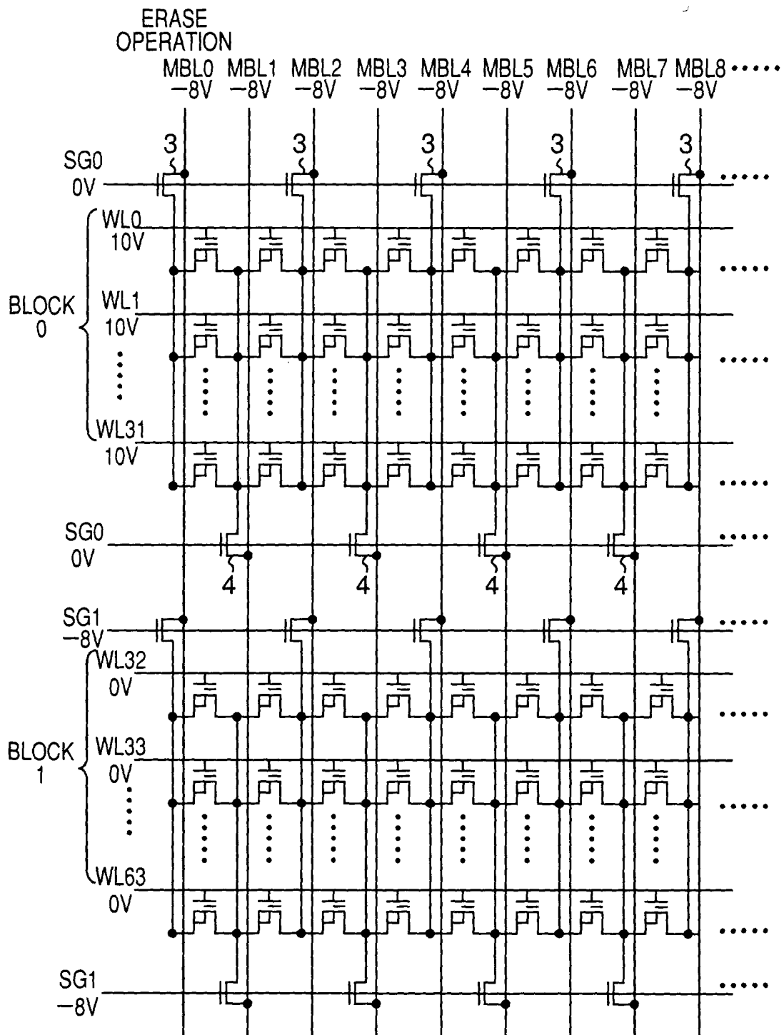
Fig.11 PRIOR ART
