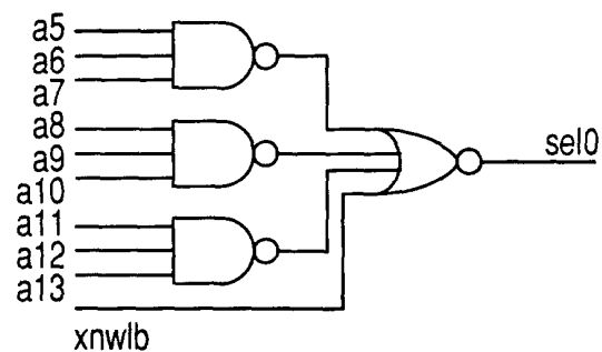
Fig.17 PRIOR ART
