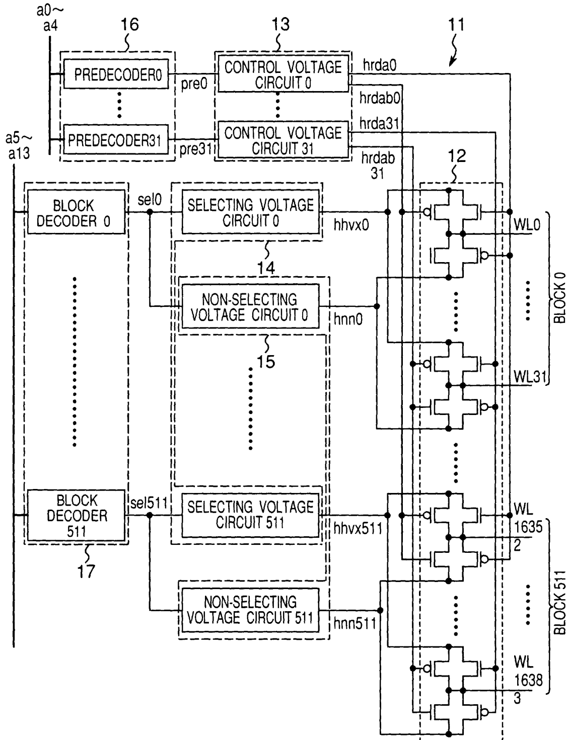
Fig.12 PRIOR ART
