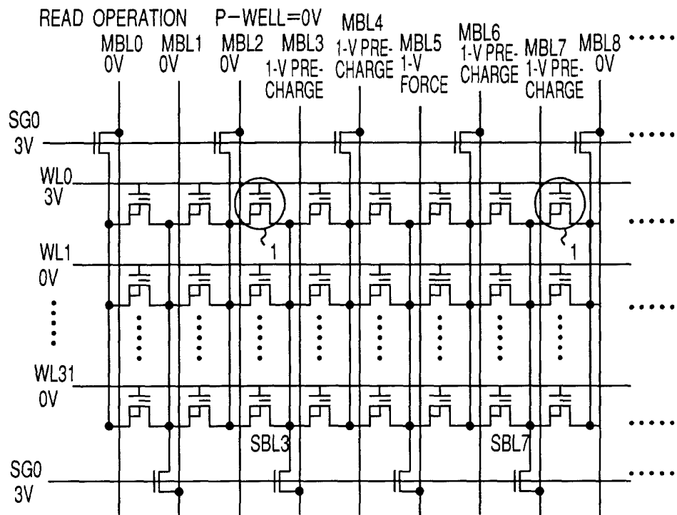
Fig.9 PRIOR ART
