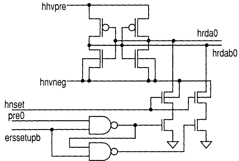
Fig.13 PRIOR ART
