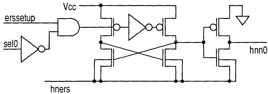
Fig.15 PRIOR ART
