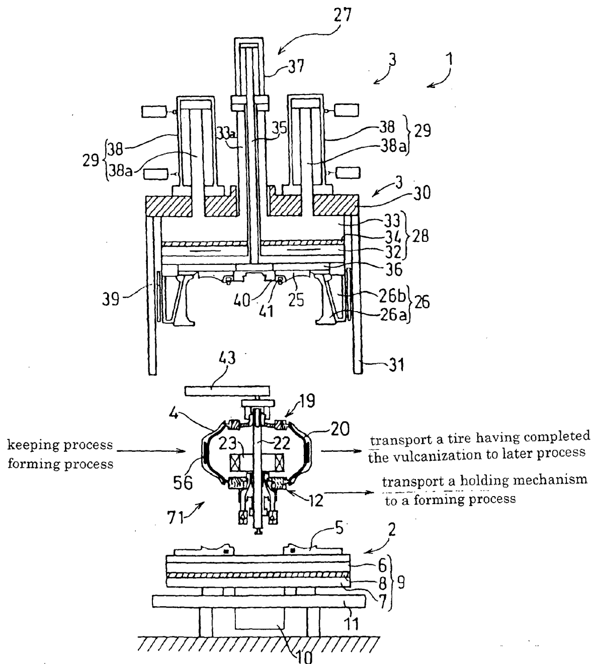
Fig. 3 vulcanizing process
