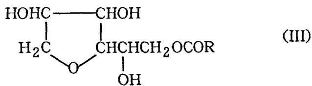
1,4-Sorbitan ester
