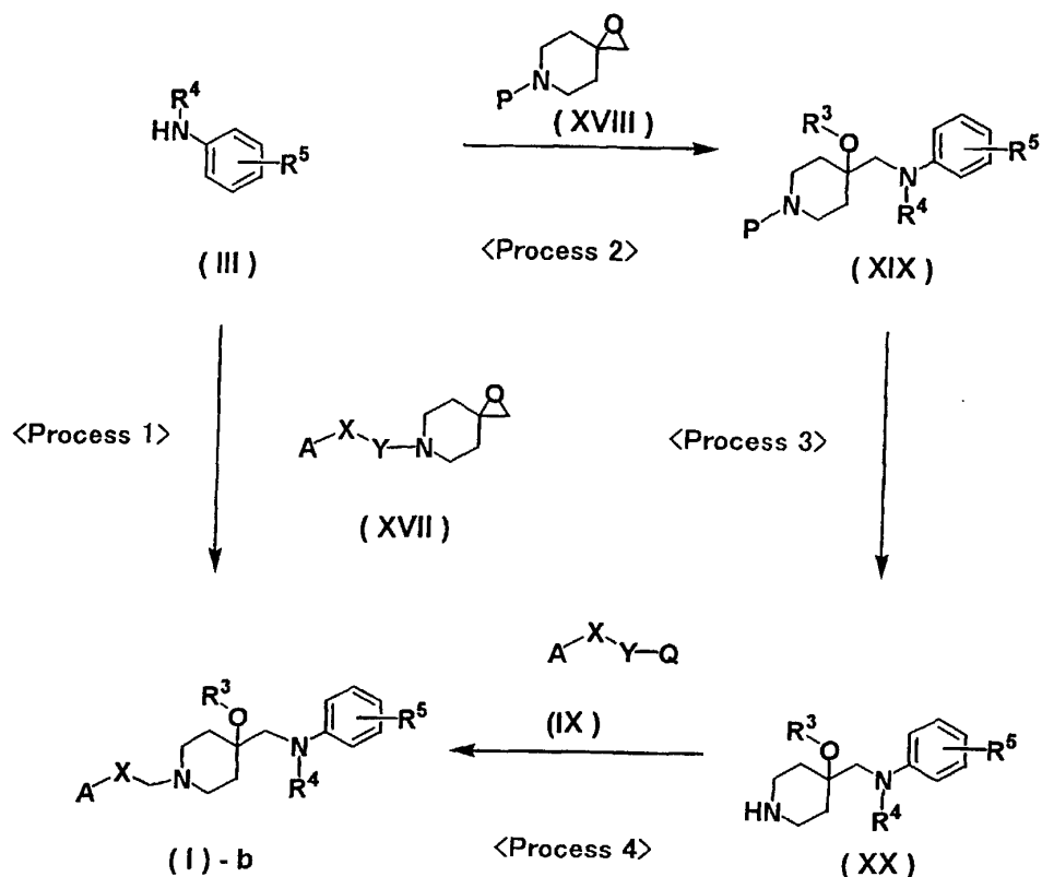
Reaction Scheme 4
