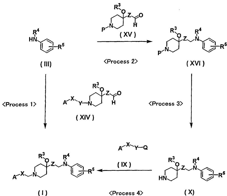
Reaction Scheme 3
