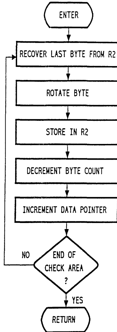
FIG 27J FIO DOWN LD/VXRAM/SKIP
