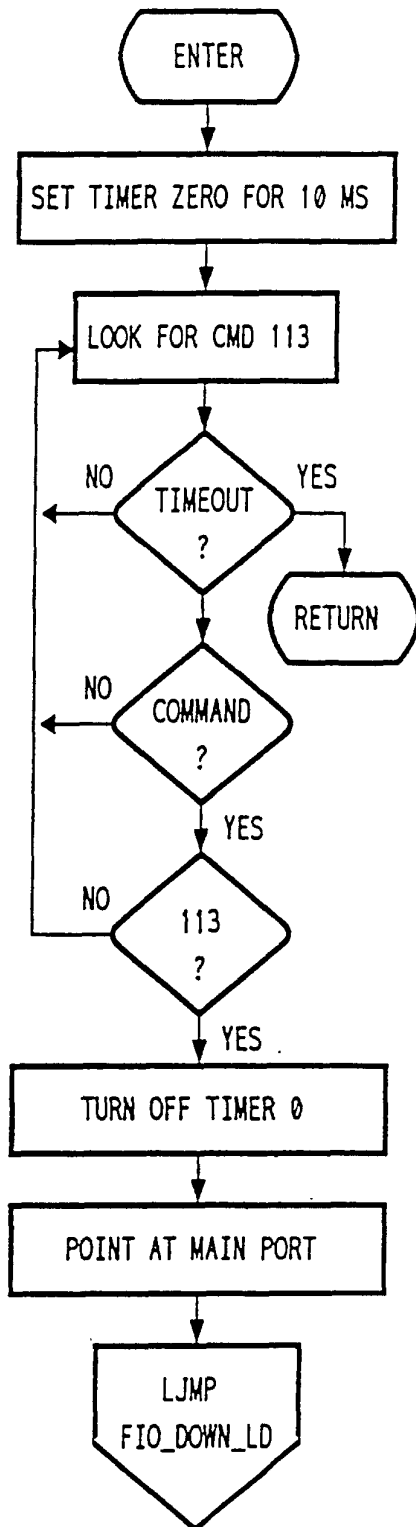
FIG 27A MY SIDE RCV/MAIN
