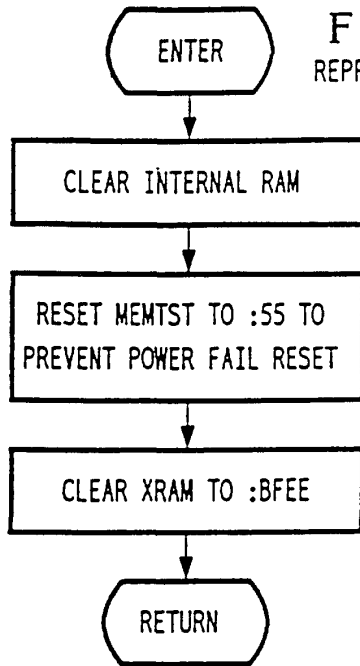
FIG 27I FIO DOWN LD/OLD PROGRAM
