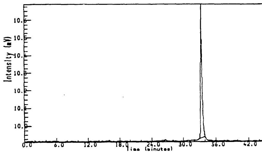
HPLC Chromatogram of Example 1 of this application using Method 1.
