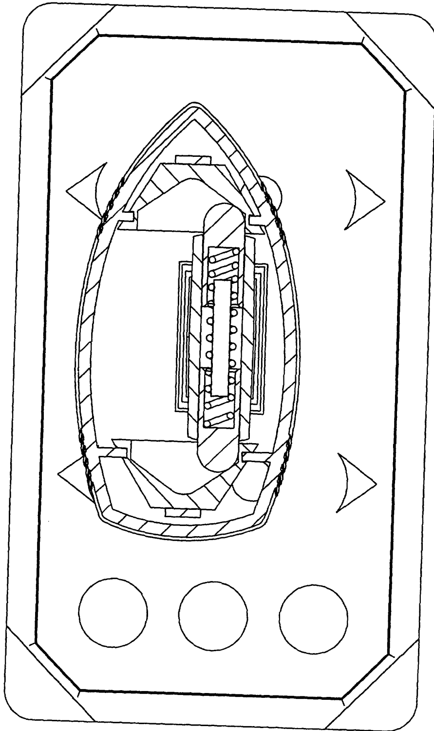
SECTION B-B
