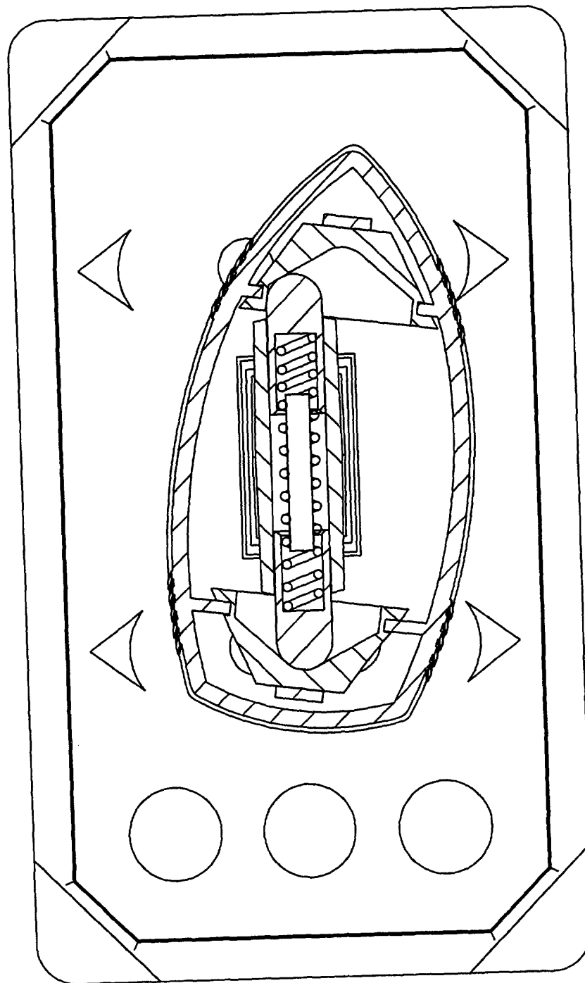
SECTION B-B
