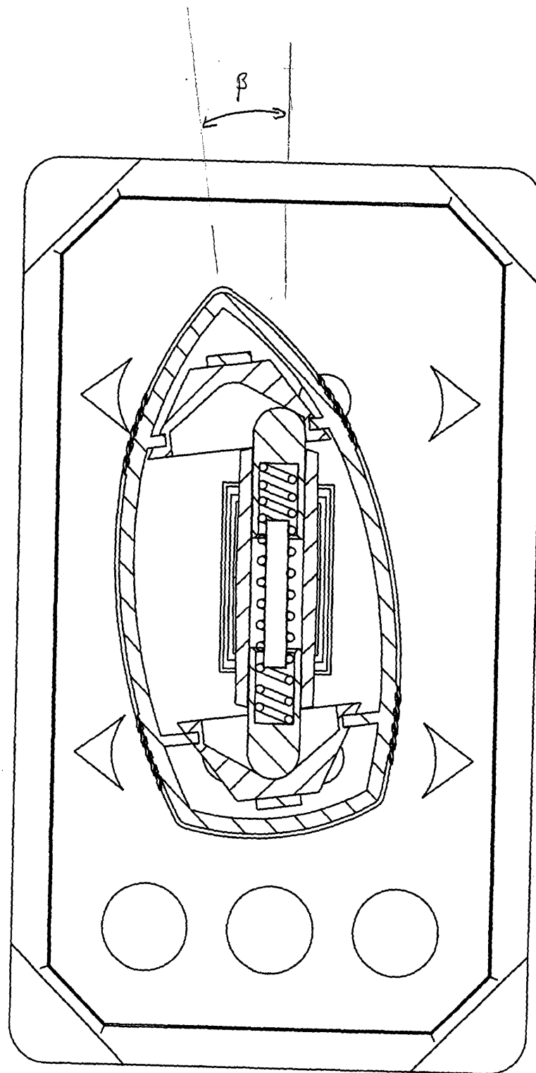
SECTION B-B
