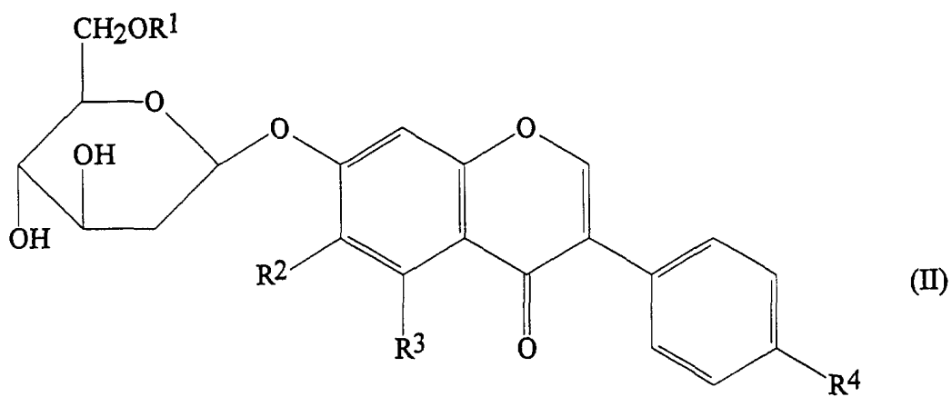
Formula (II) - Isoflavone conjugate or isoflavone glucoside
