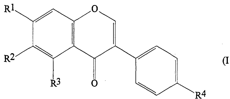
Formula (I) - Aglucone isoflavone
