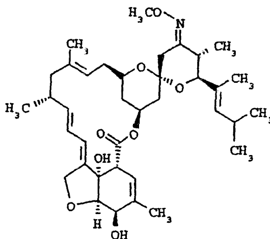
moxidectin (23-(O-methyloxime)-LL-F28249α).
