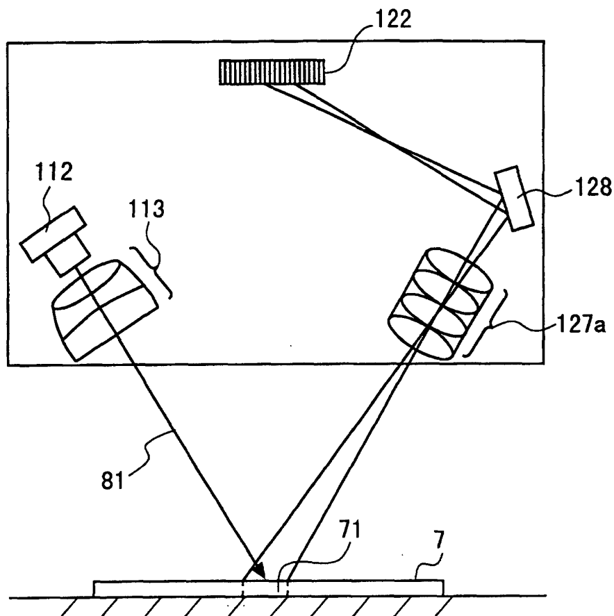
(a) diagram illustrating the observation mode using the measurement light path
