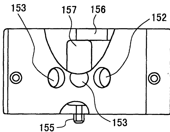
(c) bottom view
