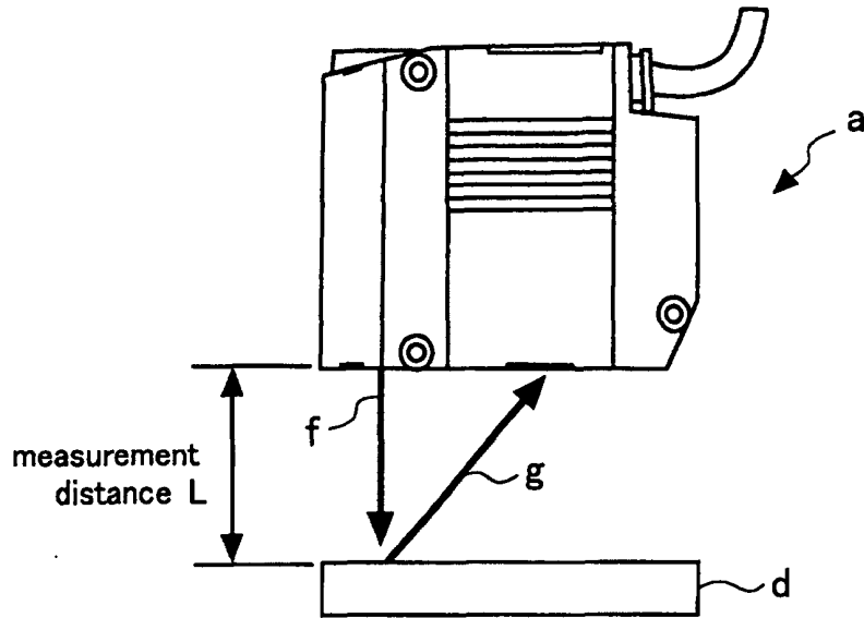
(a) light path for irregular reflective surface object
