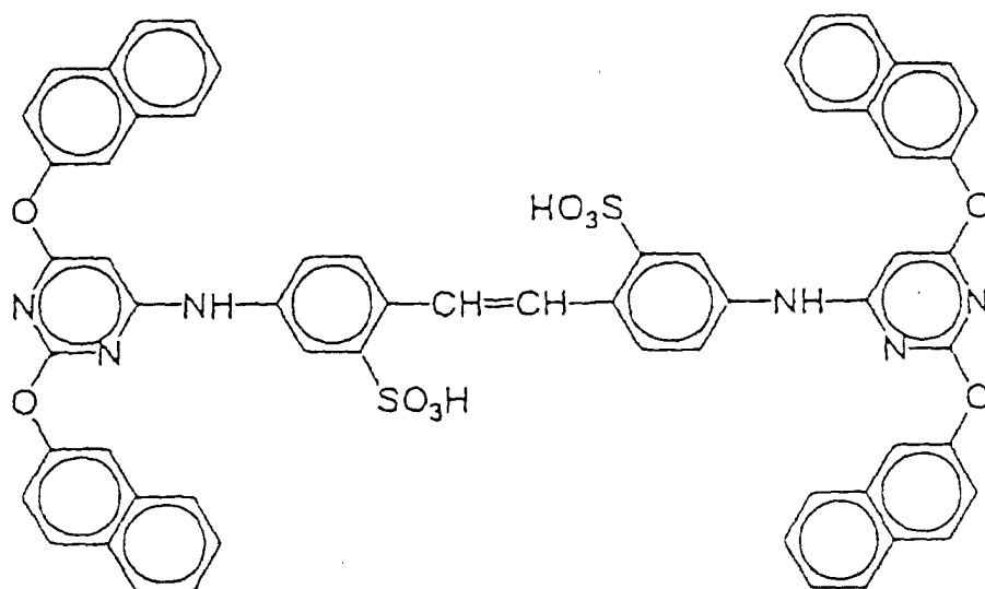
(Compound I)
