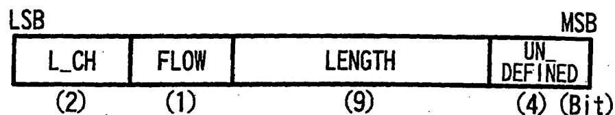
Payload Header Configuration of Multi-Slot Packet
