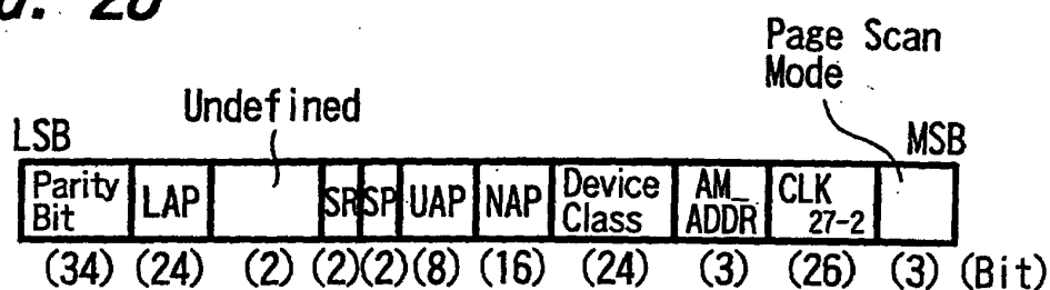
Payload of FHS Packet
