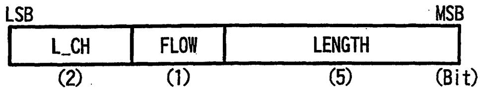
Payload Header Configuration of Single Slot Packet
