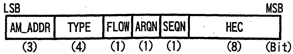
Packet Header Configuration
