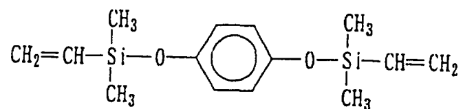
Compound No.8:
