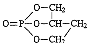
Compound No. 35:
