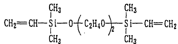
Compound No.26:
