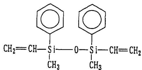
Compound No.24:
