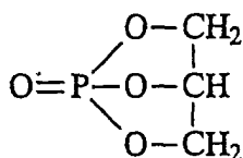
Compound No. 33:
