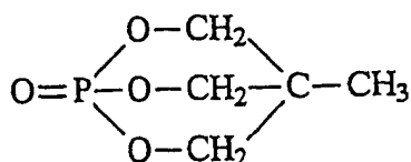
Compound No. 34:
