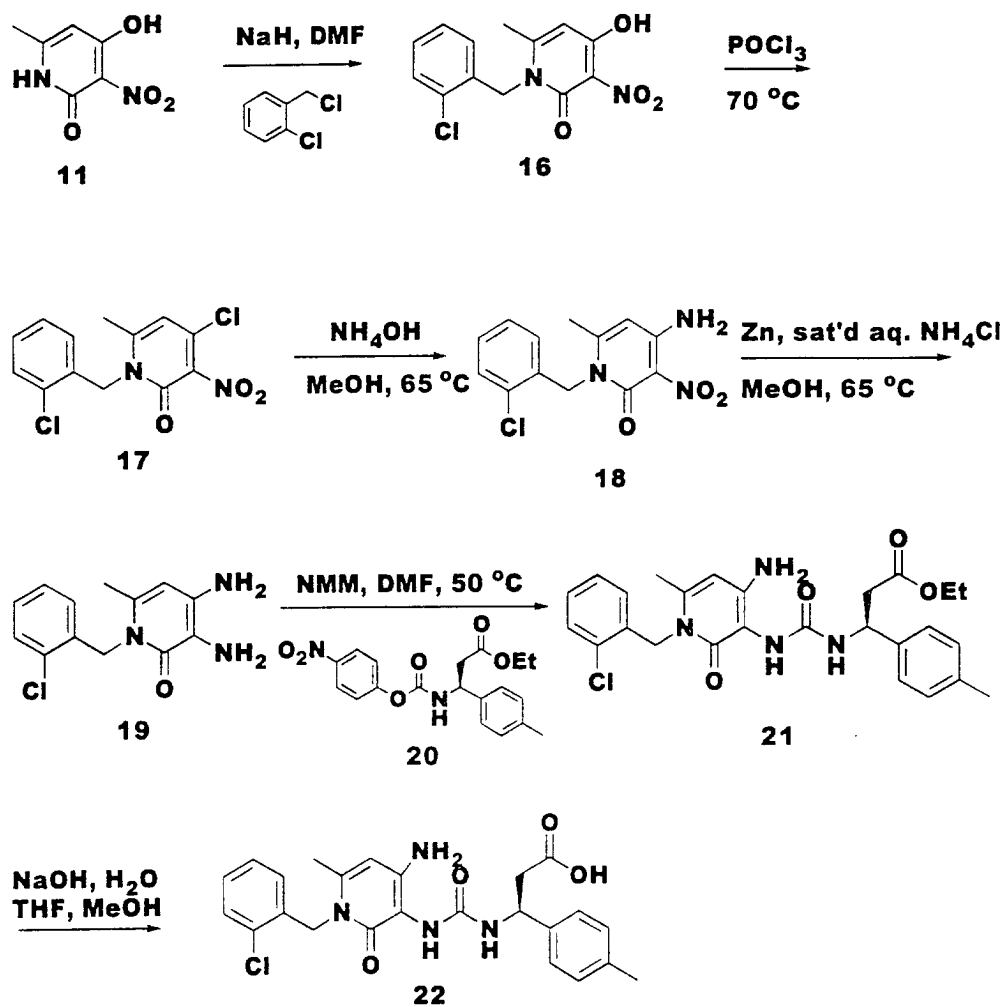
Scheme 3
