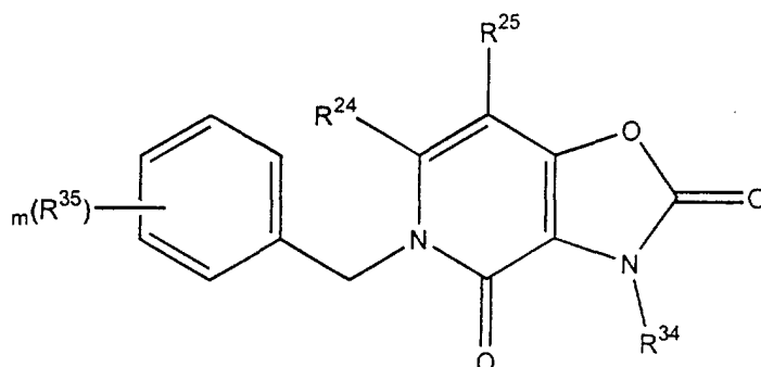
Formula VIII
