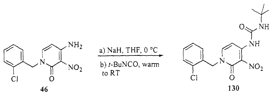
Scheme 31
