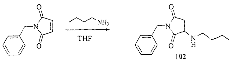
Scheme 19
