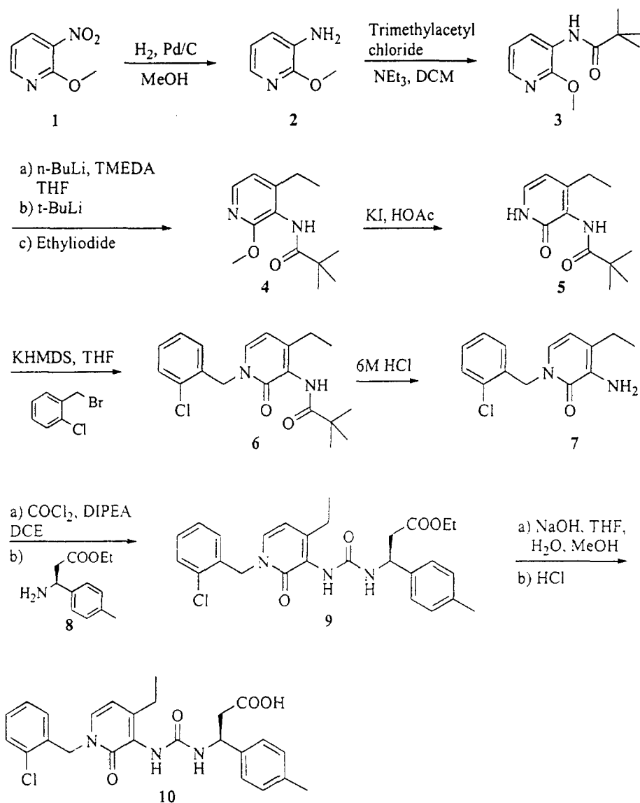
Scheme 1
