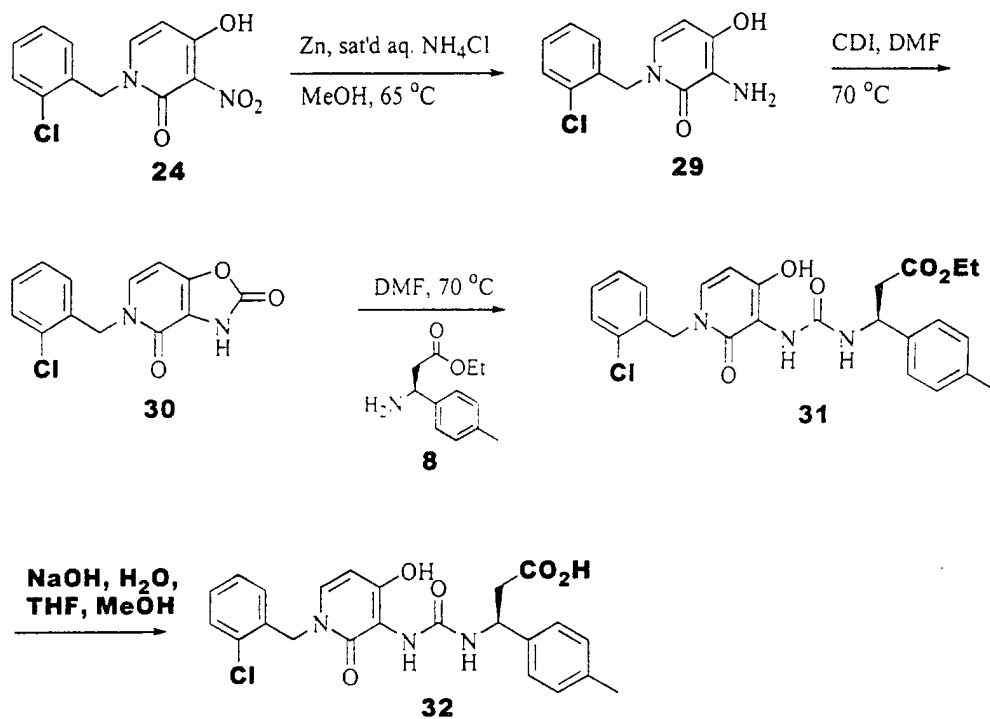
Scheme 8
