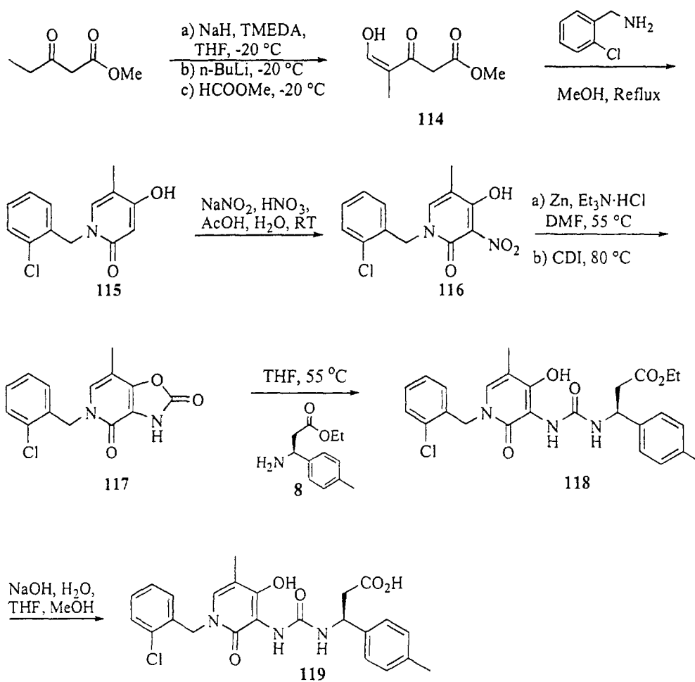
Scheme 25
