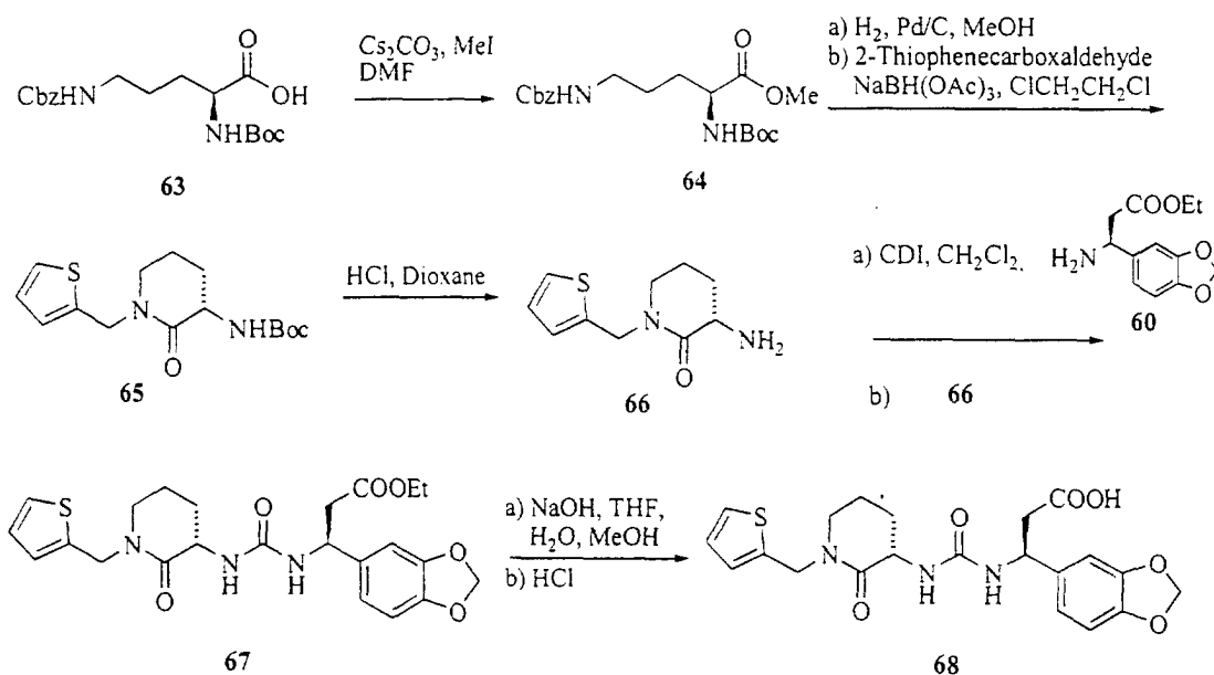
Scheme 16
