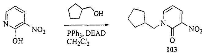
Scheme 20
