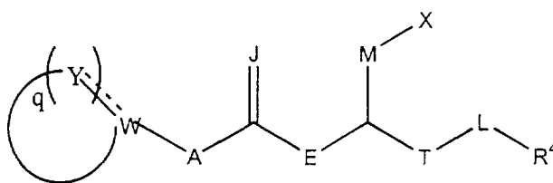
Formula I
