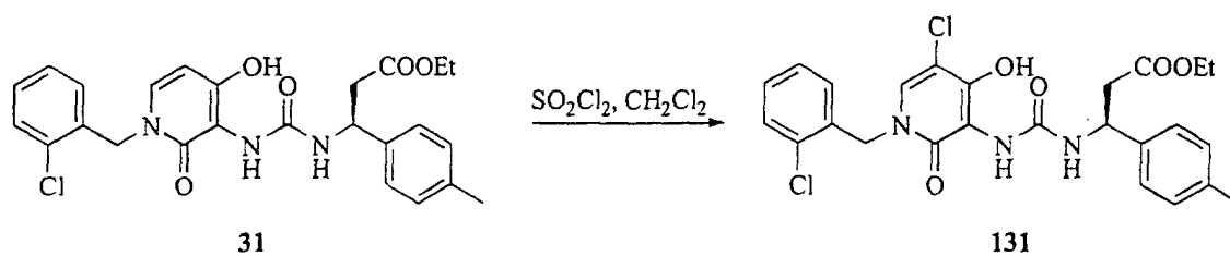
Scheme 32
