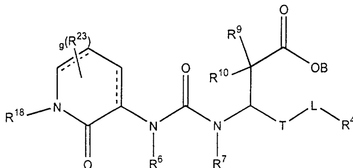
Formula IV
