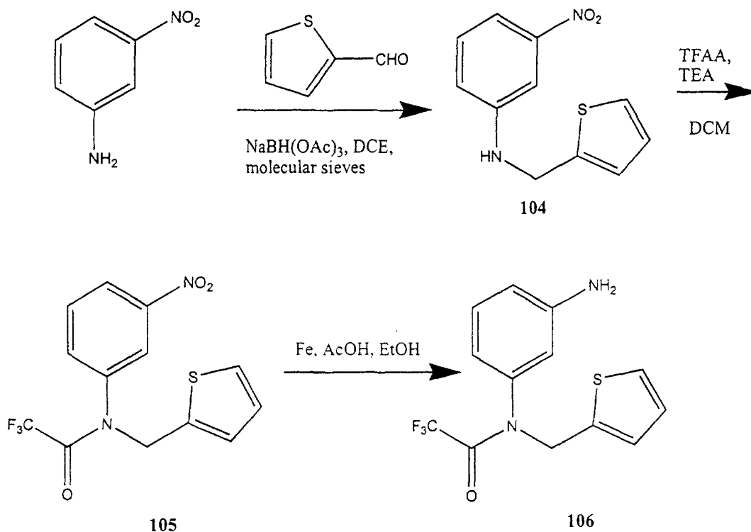
Scheme 21
