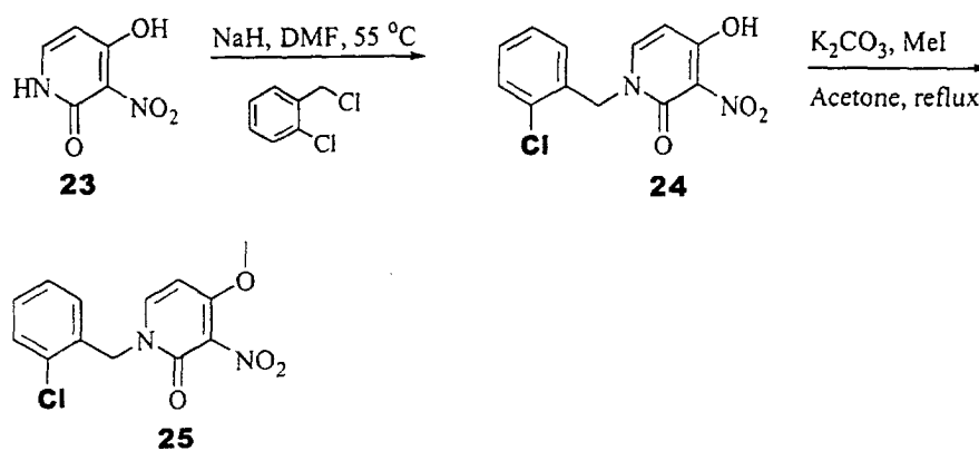
Scheme 4
