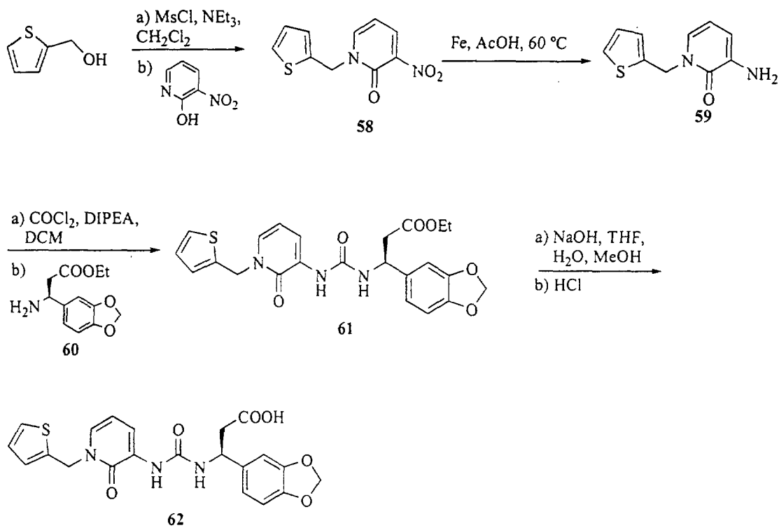
Scheme 15
