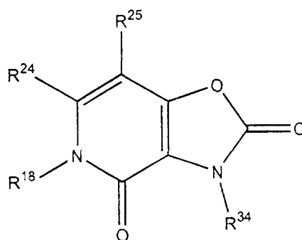
Formula VII
