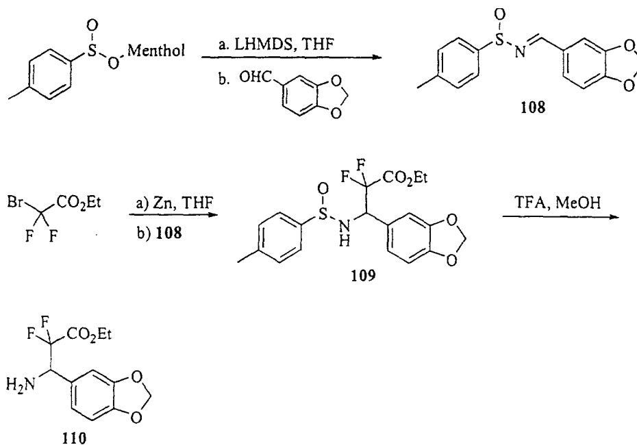
Scheme 22
