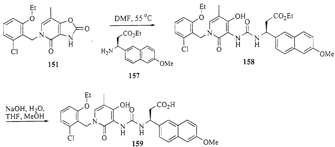
Scheme 38
