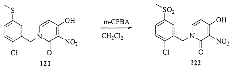
Scheme 27
