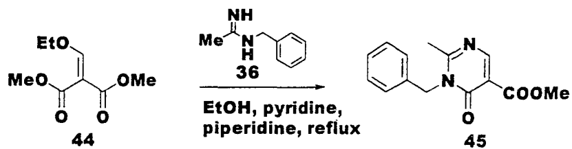
Scheme 11
