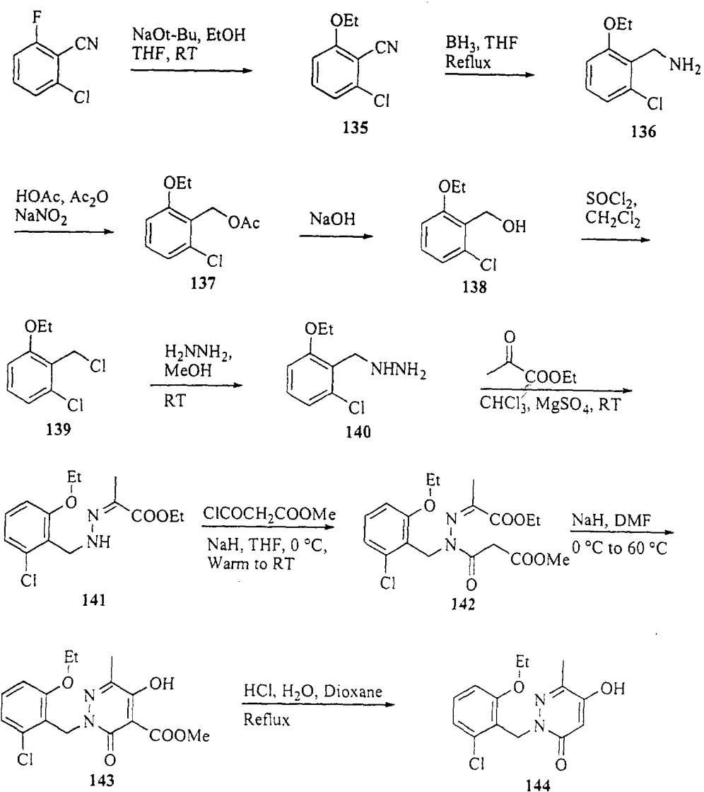
Scheme 34
