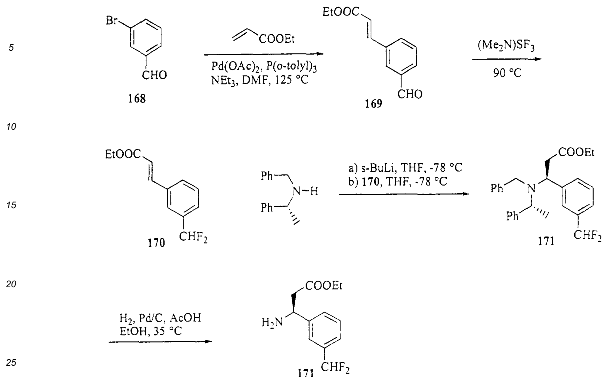
Scheme 42
