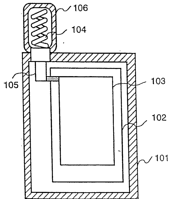
Fig.14 CONVENTIONAL ART
