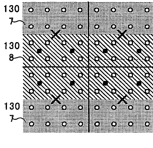
FIG. 14D DEMODULATION OF S3 IS IMPOSSIBLE
