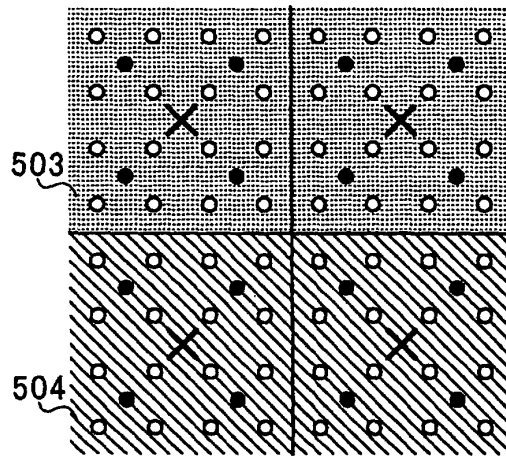
FIG. 6B DEMODULATION OF S1 IS POSSIBLE
