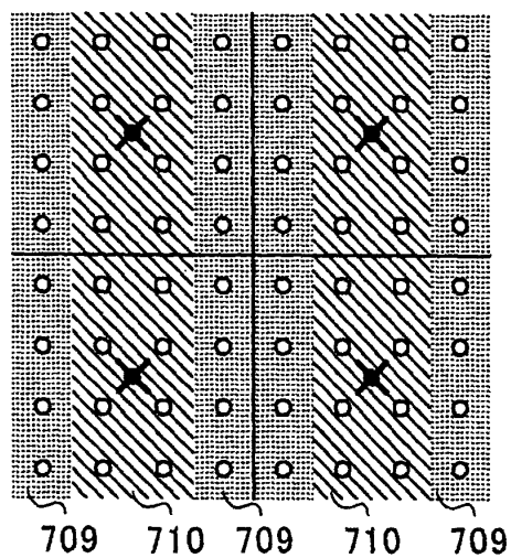
FIG. 8E DEMODULATION OF S4 IS IMPOSSIBLE
