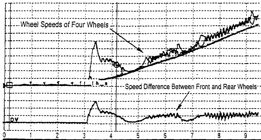
Wheel Speed Waveforms When at Grip Limit
