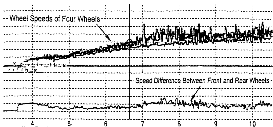
Wheel Speed Waveforms When Travelling on Poor Road
